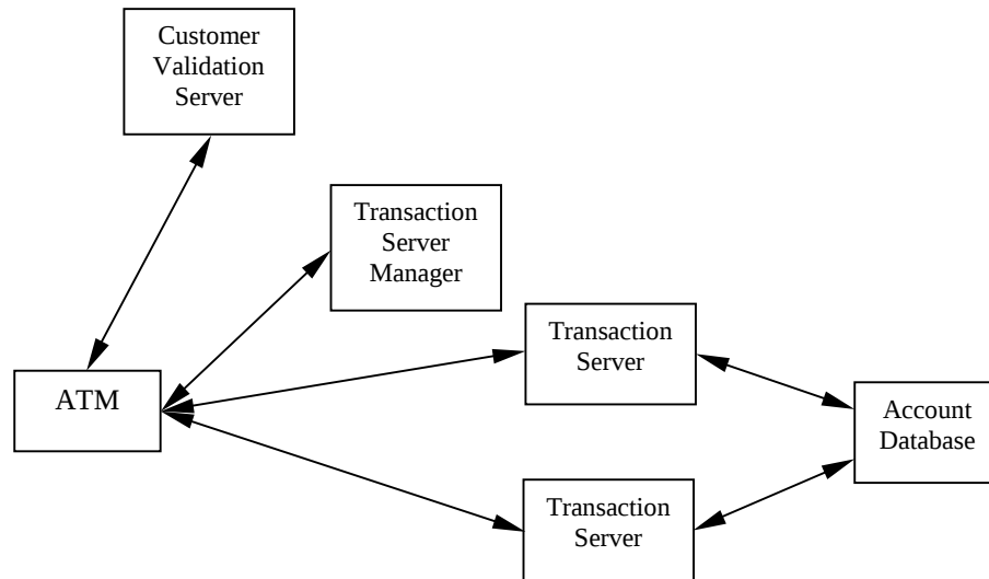
Figure 4.1 The Bank ATM System
