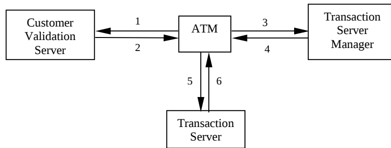
Figure 5.28 The Bank ATM Example
