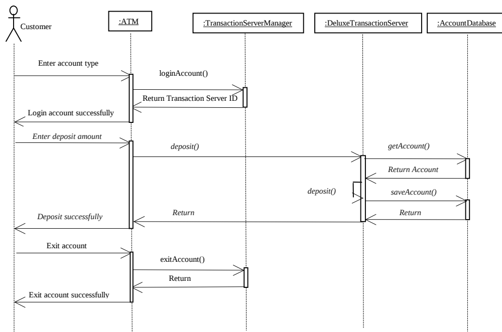
Figure 4.2 The Sequence Diagram of Deposit Money in the ATM System
