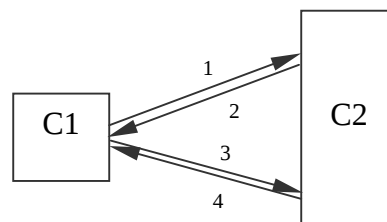
Figure 5.24 The Partial Sequential Composition of Two Synchronous Two-Way Invocation-Based Communication Patterns (Pattern No. 23)
