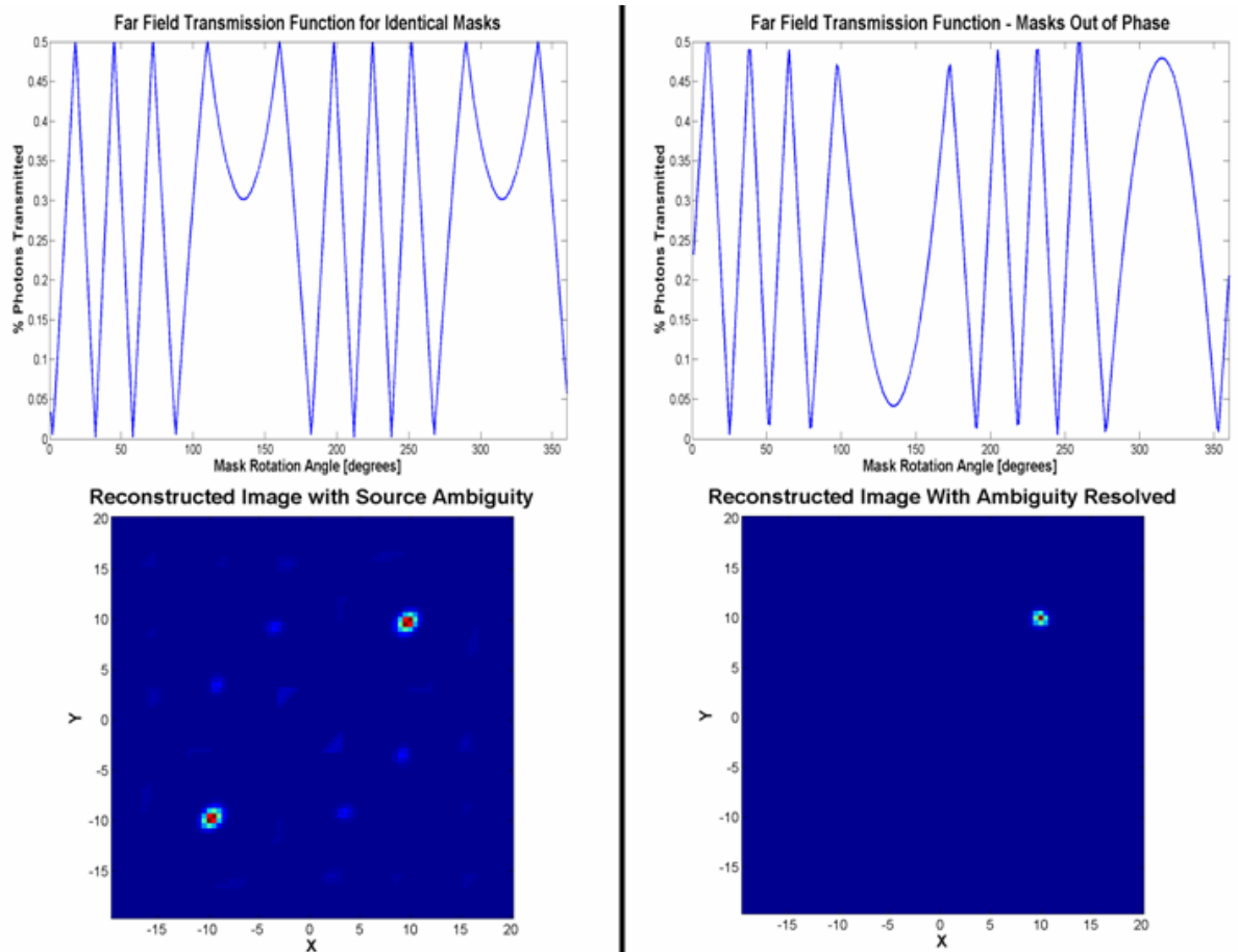
Figure 3-3. When the RMC masks are symmetric (left panels) the 180^\circ ambiguity is apparent. When the masks are made asymmetric (right panels) the ambiguity can be resolved with a single measurement. The cost of making the masks asymmetric is a reduction in the RMC modulation and geometric efficiency.
