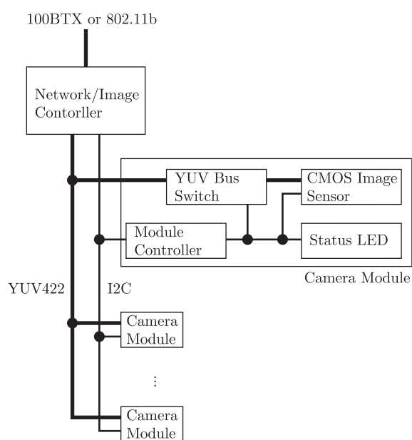
Figure 2.18: Block Diagram of the Satellite System
