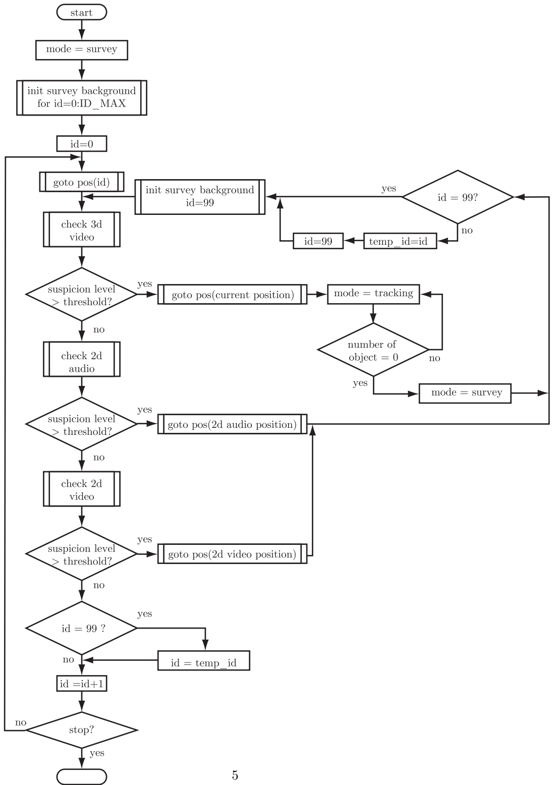
Figure 2.2: Mode Transition of the System
