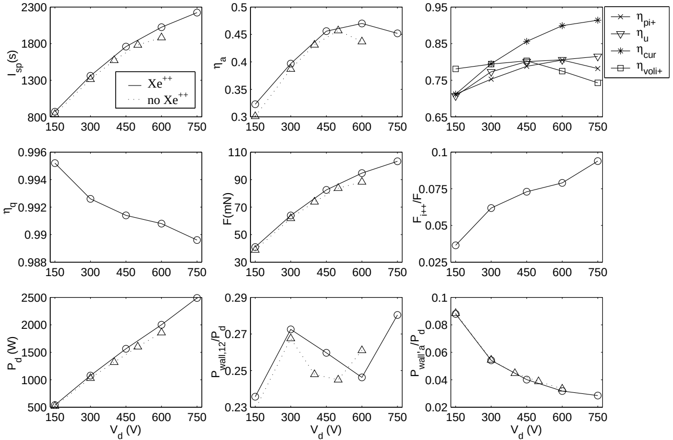
Figure 6.8: Variation of main operation parameters when varying the discharge potential V_d . P_{wall,12} and P_{wall,a} represent total energy losses to inner and outer walls and to the anode.
