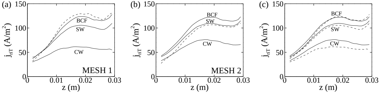
Figure 4.5: Axial profiles of ion current density to the inner wall for (a) mesh 1 and (b) mesh 2. In figures (a) and (b), the dashed line is the theoretical Bohm flux ( j_{\text{Bohm}} ) for SW and the corresponding mesh. (c) Comparison of sensitivities to the mesh size of CW, SW and BCF. Dashed lines represent results for mesh 1 and solid lines represent results for mesh 2.
