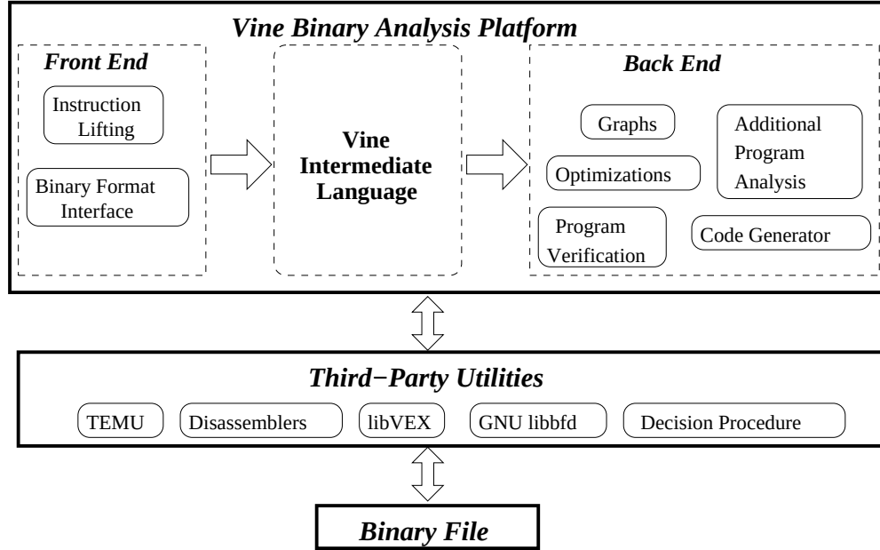
Figure 2.3: TheVine binary analysis architecture and components. Vine is divided into a front-end, which is responsible for lifting instructions to the Vine IL, and a platform-independent back-end for analyses.
