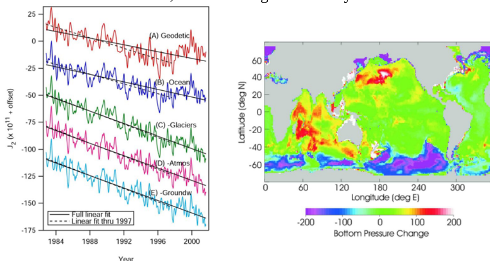
Figure 4: (Left) Earth oblateness ( J_2 ) observations (red curve labeled A) and residuals obtained by successive removal of the source terms. Removal of the ocean estimate (blue curve labeled B) accounts for 42% of the nonlinear change in J_2 . (Right) Change of average ocean bottom pressure between 1996-97 and 1999-2000. (Both from Dickey et al. (2002).) [Ocean bottom pressure decreases in the Southern Ocean and increases in the Indian Ocean and the North Pacific Ocean.]
