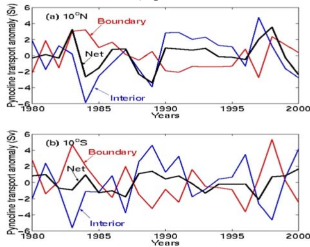
Figure 2: Anomaly time series of tropical-subtropical meridional pycnocline transport in the Pacific Ocean along 10°N (top) and 10°S (bottom). Transport in the low latitude boundary layer (red) is out of phase with and partially compensate that in the interior (blue). (From Lee et al. (2003).)
