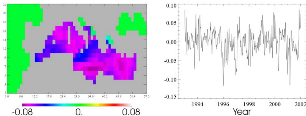
Figure 3: (Left) First empirical orthogonal function (EOF) of non-seasonal Mediterranean Sea sea level variability, (Right) Amplitude time-series of the first EOF. (From Fukumori (2003b).) [The first EOF is nearly uniform over the Mediterranean Sea with variability at periods of 10s of days to several months.]
