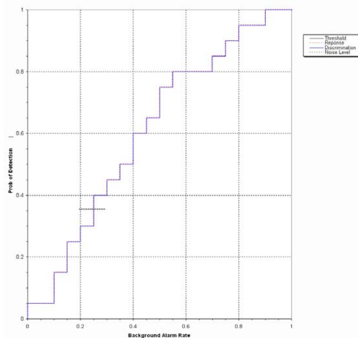
Figure 5. MAG G823/sling blind grid probability of detection for response and discrimination stages versus their respective probabilities of background alarm for all ordnance larger than 20 mm.
