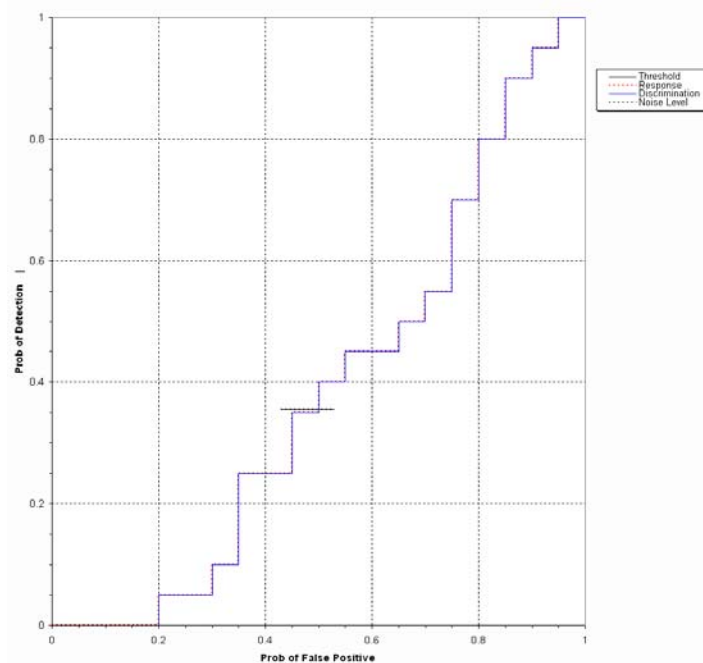
Figure 4. MAG G823/sling blind grid probability of detection for response and discrimination stages versus their respective probability of false positive for all ordnance larger than 20 mm.
