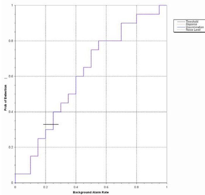
Figure 3. MAG G823/sling blind grid probability of detection for response and discrimination stages versus their respective probability of background alarm over all ordnance categories combined.
