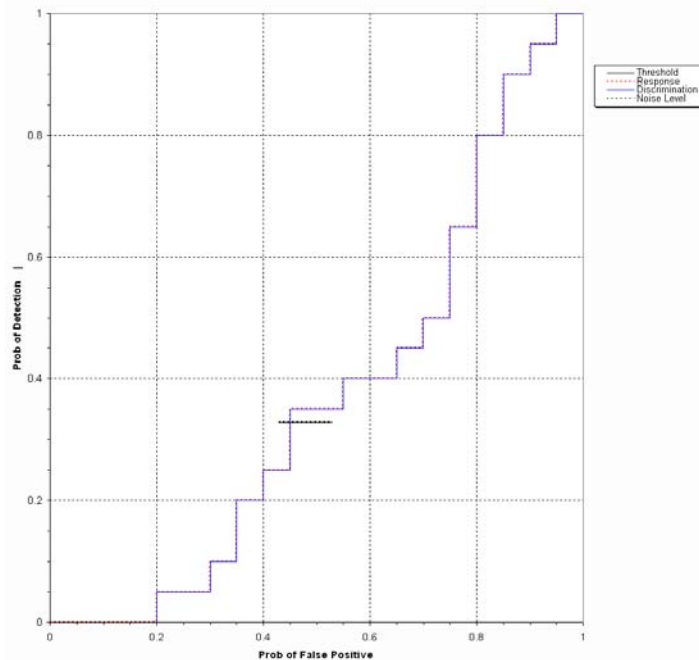
Figure 2. MAG G823/sling blind grid probability of detection for response and discrimination stages versus their respective probability of false positive over all ordnance categories combined.
