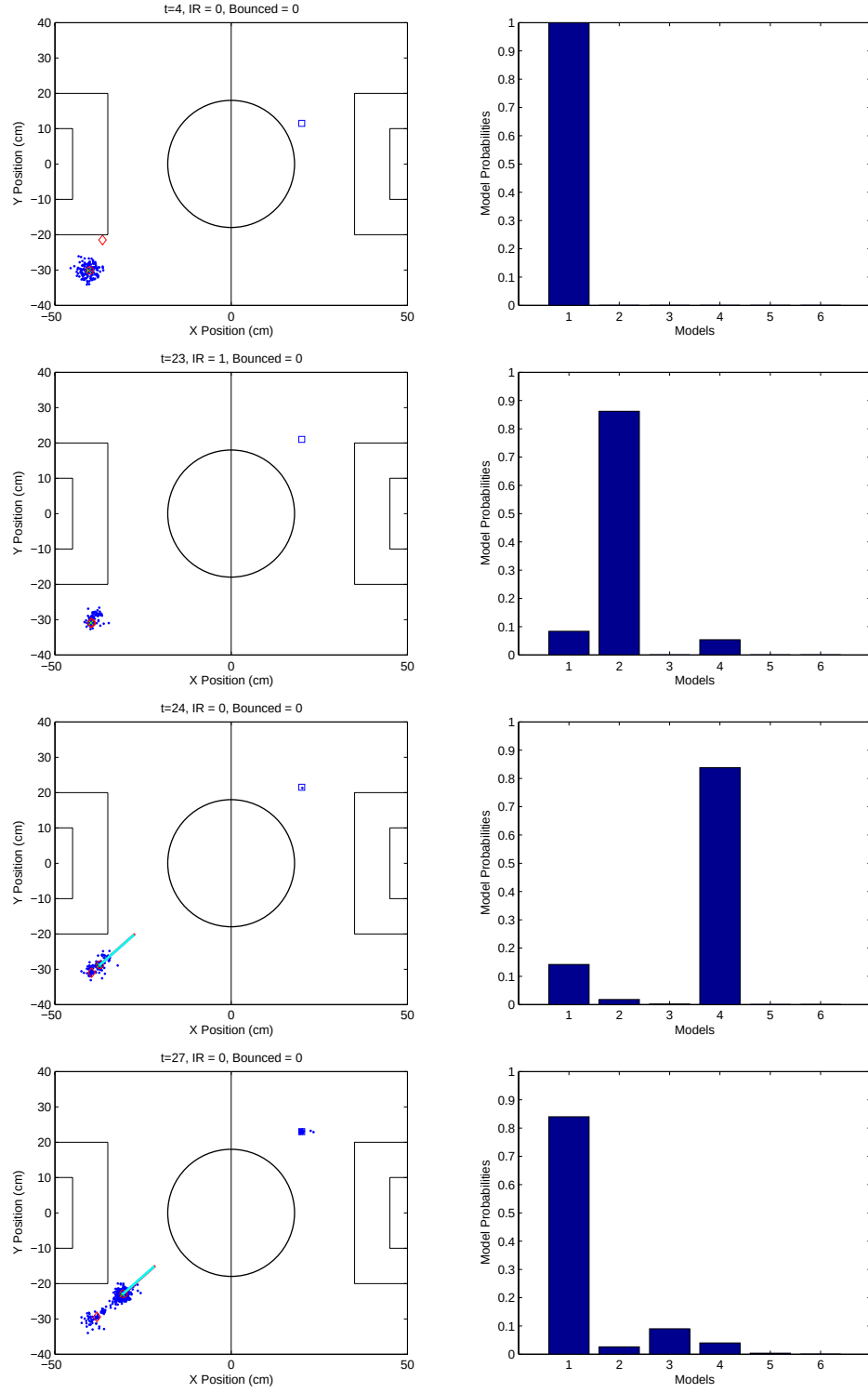
Figure 5.7: The snapshots of the particle cloud and the model probabilities at t = 4, 23, 24 , and 27.
