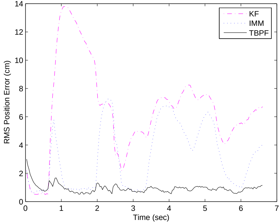
Figure 4.10: RMS position error versus time
