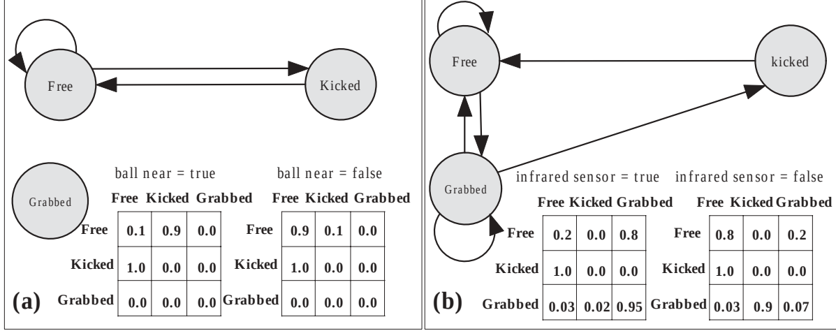
Figure 4.3: Ball motion model. Each node is a single model. The tables list the transition probability between any two single models. (a) Ball motion model based on tactic chase_ball . (b) Ball motion model based on tactic grab_and_kick .
