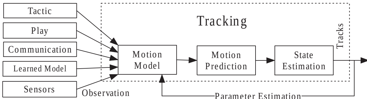
Figure 2.1: Top-level structure of our proposed approach
