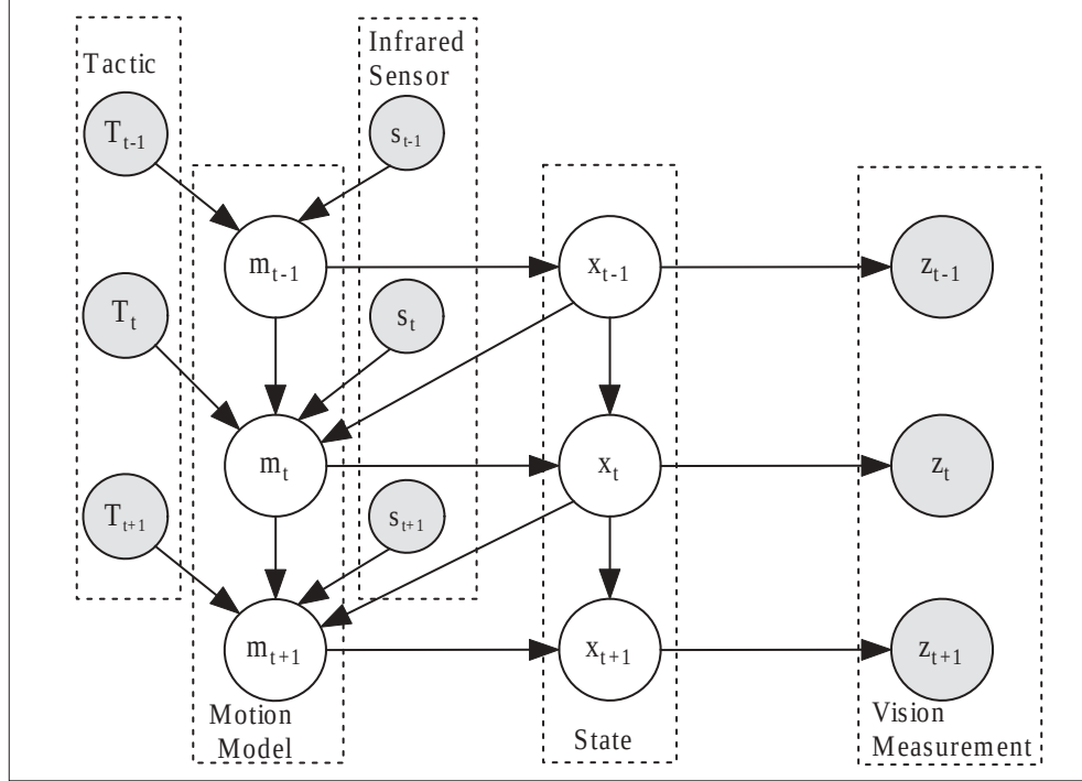
Figure 4.4: A dynamic bayesian network for tactic-based object tracking. Filled circles represent deterministic variables which are observable or are known as the tactic that the robot is executing.
