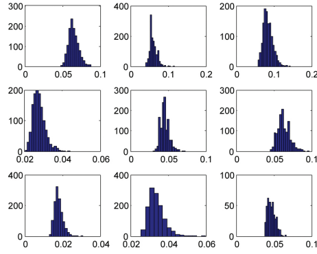
Figure 14: Histograms of closeness centralization by network size and density First row is N = 250 , second N = 50 , and the last N = 1000 , with first column d = 1\% , second 2\% , and third 5\%
