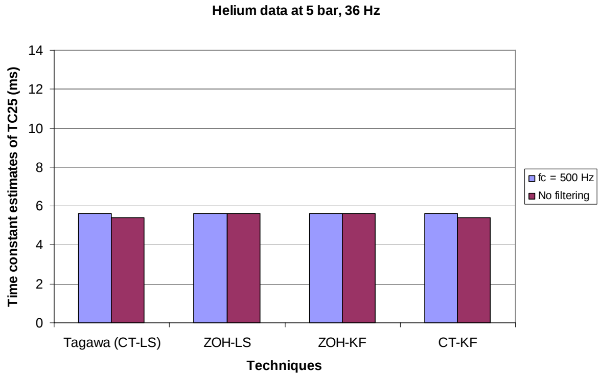
Figure 6 Comparison of different two-thermocouple techniques. Helium gas, 5 bar fill pressure, 10 mm stroke at 36 Hz.
