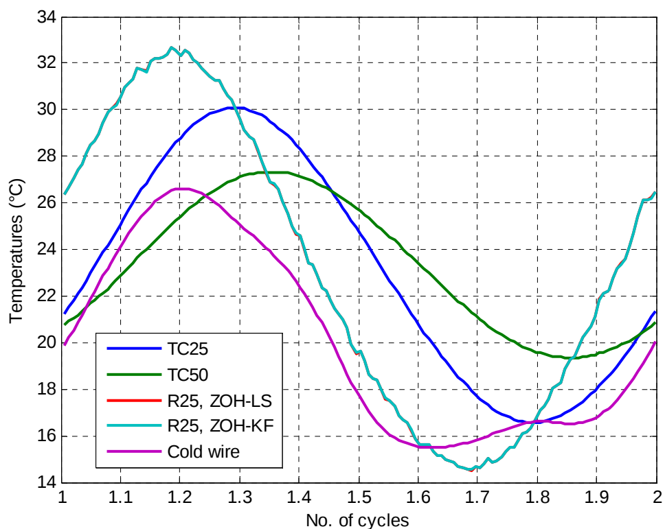
Figure 14 Comparison of the raw and compensated thermocouple and cold wire temperatures. The sampling frequency was decimated to 2.5 kHz. Helium gas, 5 bar fill pressure, 10 mm stroke at 18 Hz.
