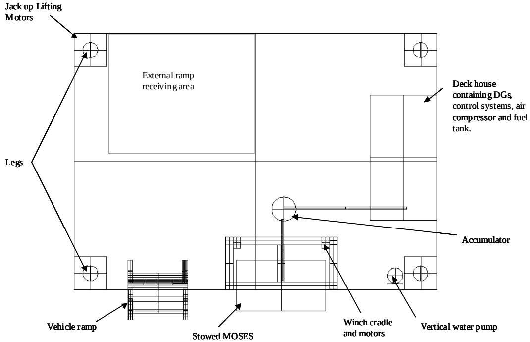
Figure 5 - Deck Plan
