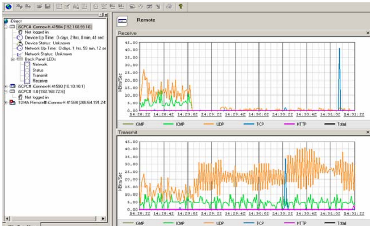
Figure 34. Shutting down of Transmissions: 14:29 (12 March 2008).
