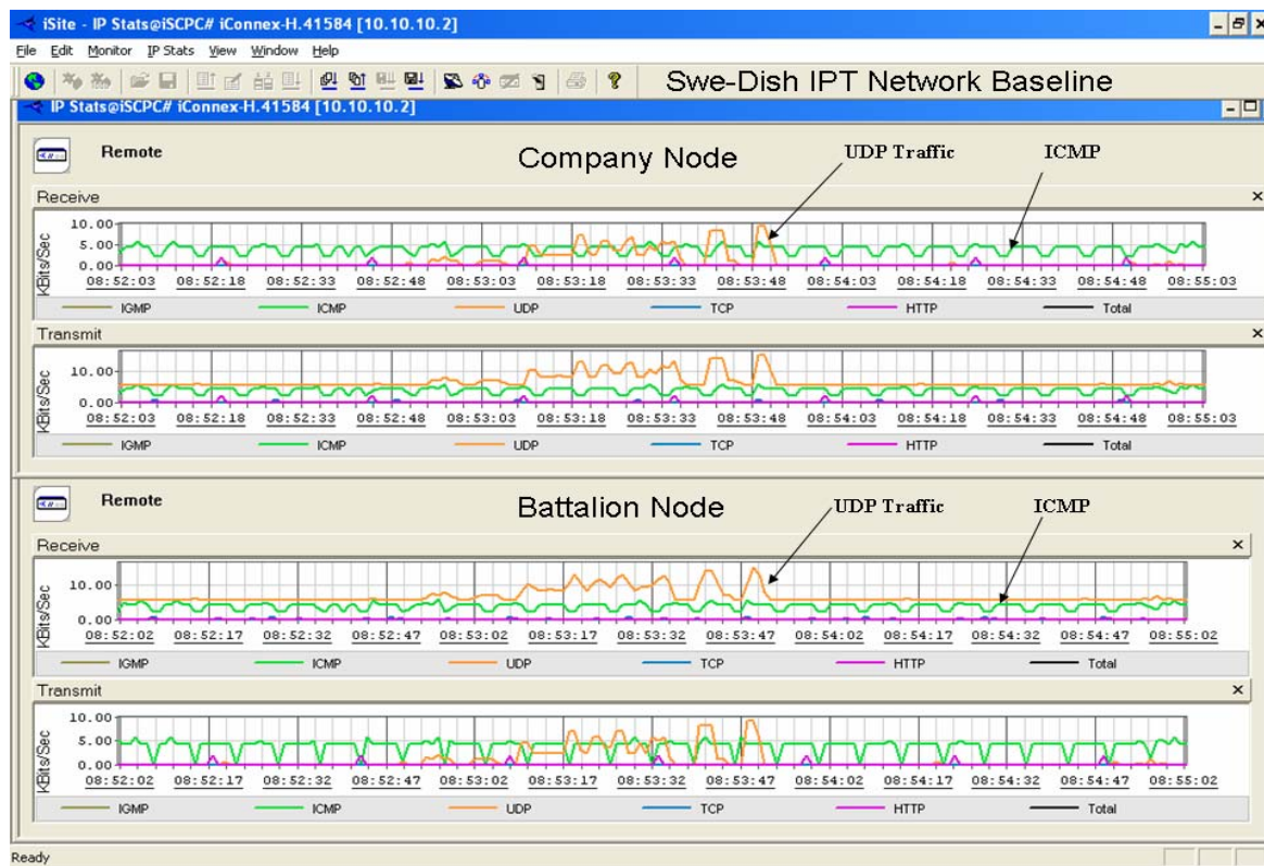
Figure 48. Baseline of Satellite Link.
