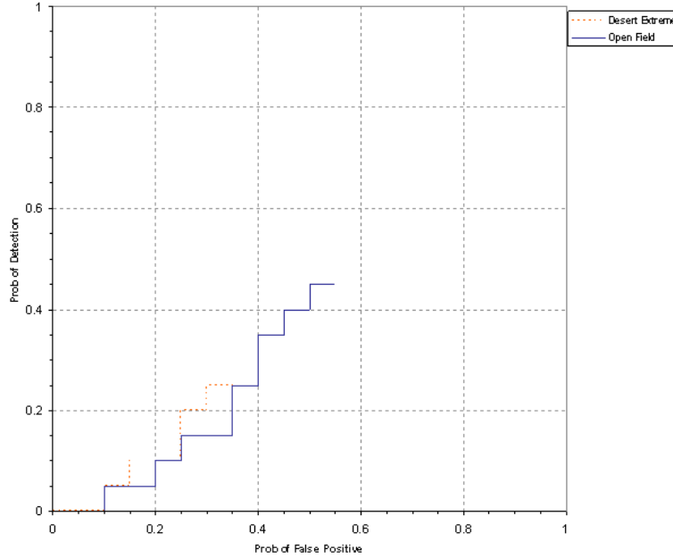
Figure 9. MAG G823/sling P_d^{\text{disc}} versus the respective P_{\text{fp}} for ordnance larger than 20 mm.
