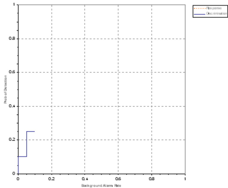
Figure 5. MAG G823/sling open field probability of detection for response and discrimination stages versus their respective background alarm rate for all ordnance larger than 20 mm.
