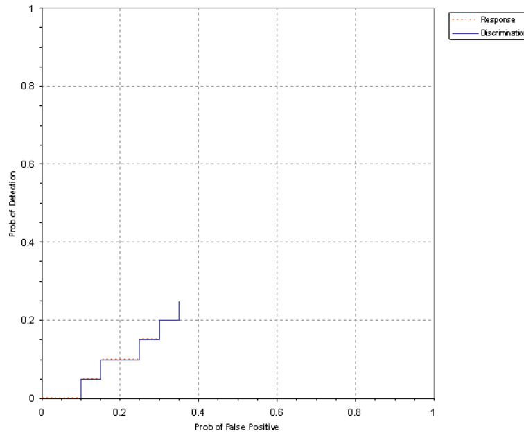
Figure 2. MAG G823/sling open field probability of detection for response and discrimination stages versus their respective probability of false positive over all ordnance categories combined.
