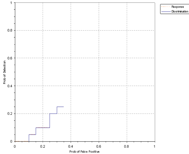
Figure 4. MAG G823/sling open field probability of detection for response and discrimination stages versus their respective probability of false positive for all ordnance larger than 20 mm.
