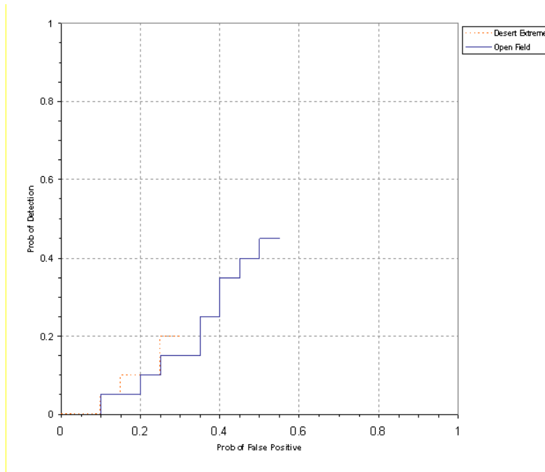
Figure 8. MAG G823/sling P_d^{\text{res}} versus the respective P_{fp} for ordnance larger than 20 mm.
