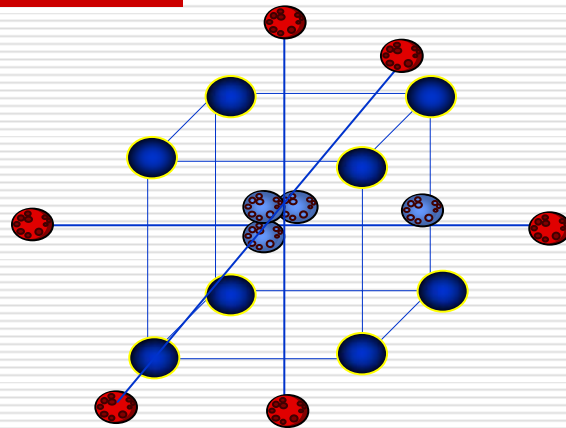
Central Composite
