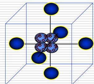
Face-Centered CCD
