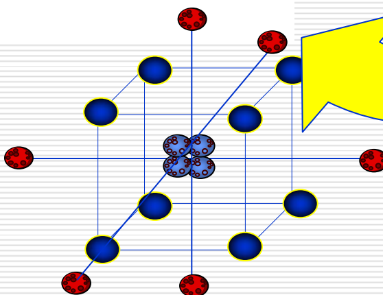
Central Composite
