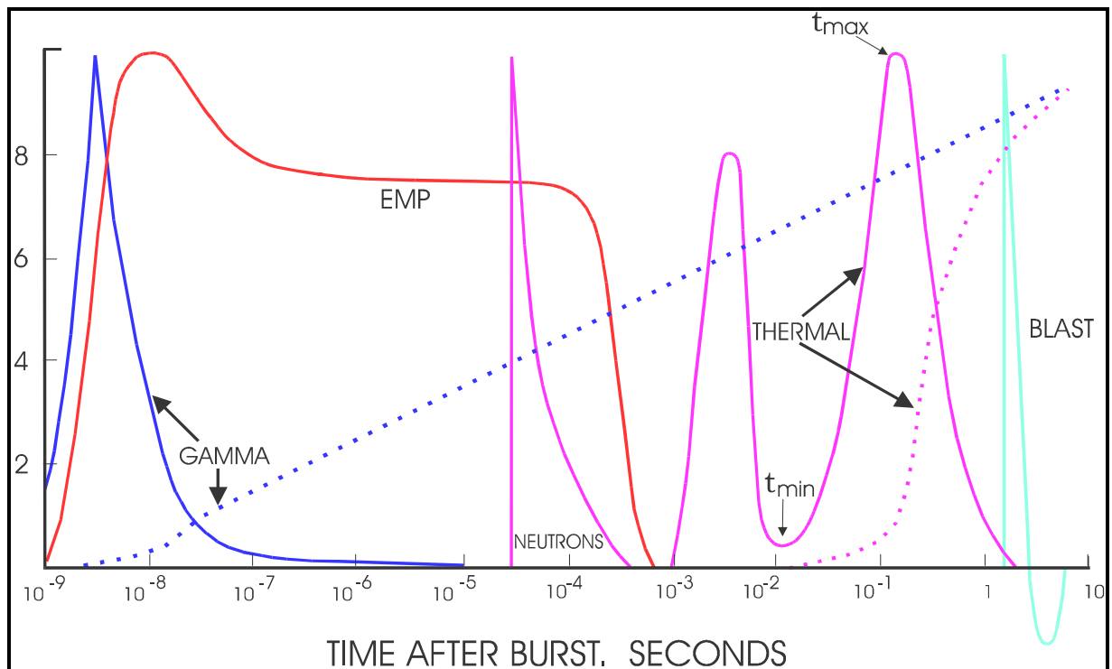
Figure D-2 Nuclear Weapon Detonation Time History
