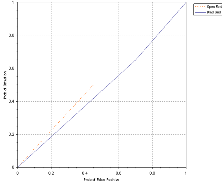
Figure 9. MAG AMOS/towed P_d^{\text{disc}} versus the respective P_{\text{fp}} for ordnance larger than 20 mm.
