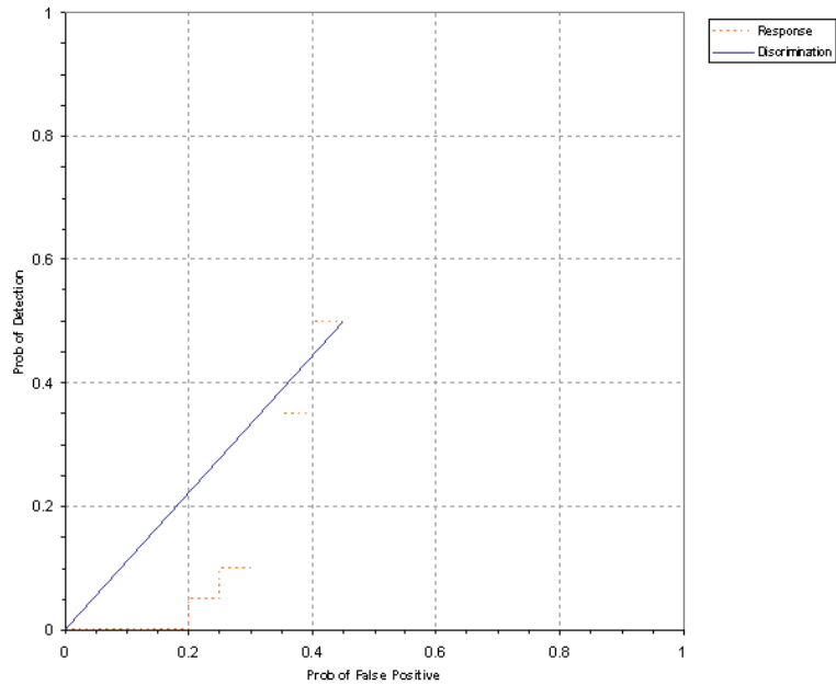
Figure 4. MAG AMOS/towed open field probability of detection for response and discrimination stages versus their respective probability of false positive for all ordnance larger than 20 mm.
