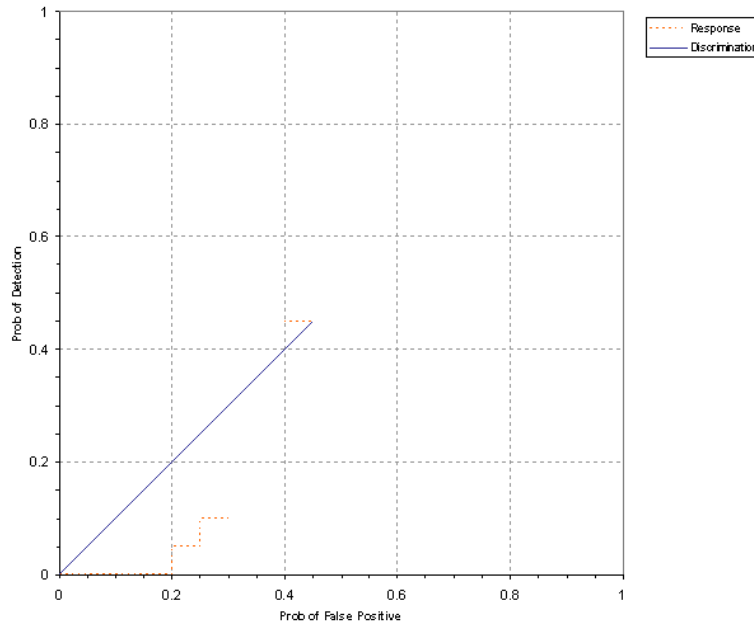
Figure 2. MAG AMOS/towed open field probability of detection for response and discrimination stages versus their respective probability of false positive over all ordnance categories combined.
