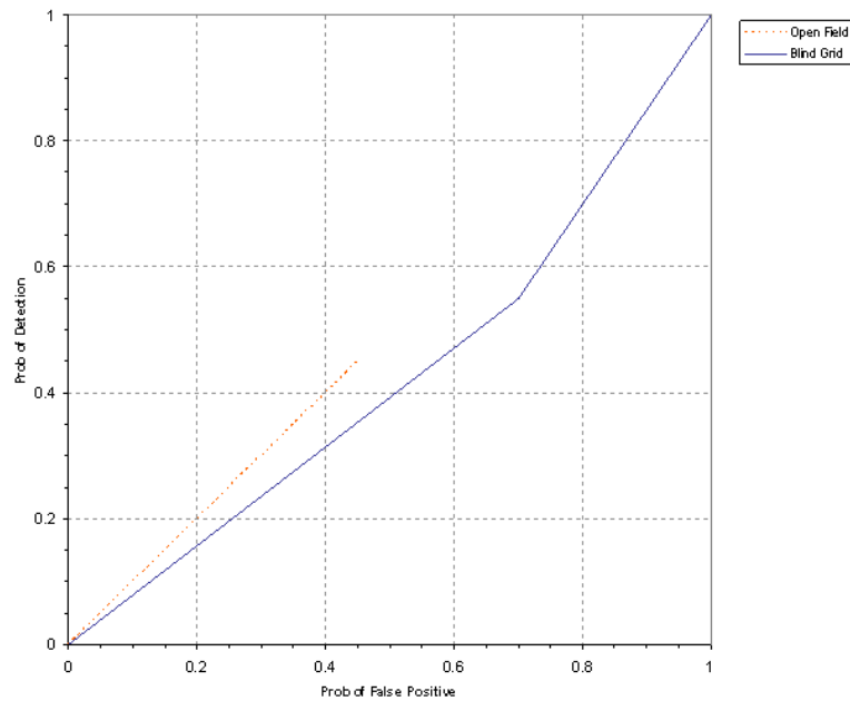
Figure 7. MAG AMOS/towed P_d^{\text{disc}} versus the respective P_{\text{fp}} over all ordnance categories combined.
