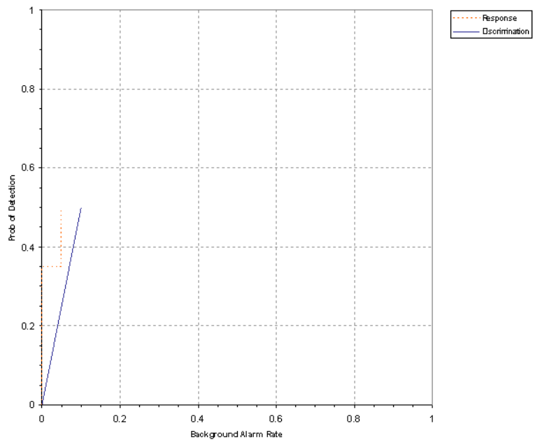
Figure 5. MAG AMOS/towed open field probability of detection for response and discrimination stages versus their respective background alarm rate for all ordnance larger than 20 mm.
