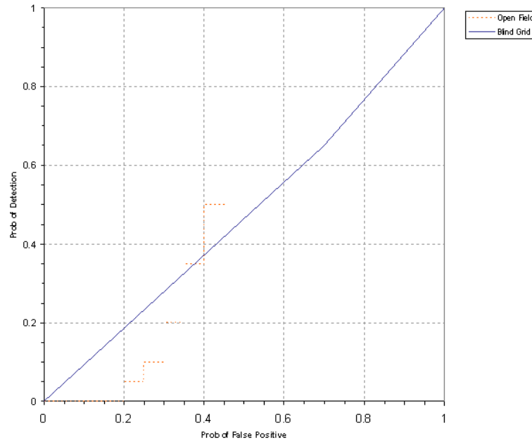
Figure 8. MAG AMOS/towed P_d^{\text{res}} versus the respective P_{\text{fp}} for ordnance larger than 20 mm.
