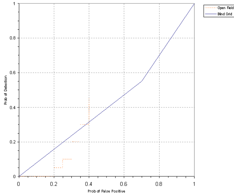
Figure 6. MAG AMOS/towed P_d^{\text{res}} stages versus the respective P_{\text{fp}} over all ordnance categories combined.
