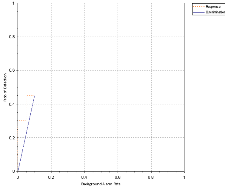
Figure 3. MAG AMOS/towed open field probability of detection for response and discrimination stages versus their respective background alarm rate over all ordnance categories combined.
