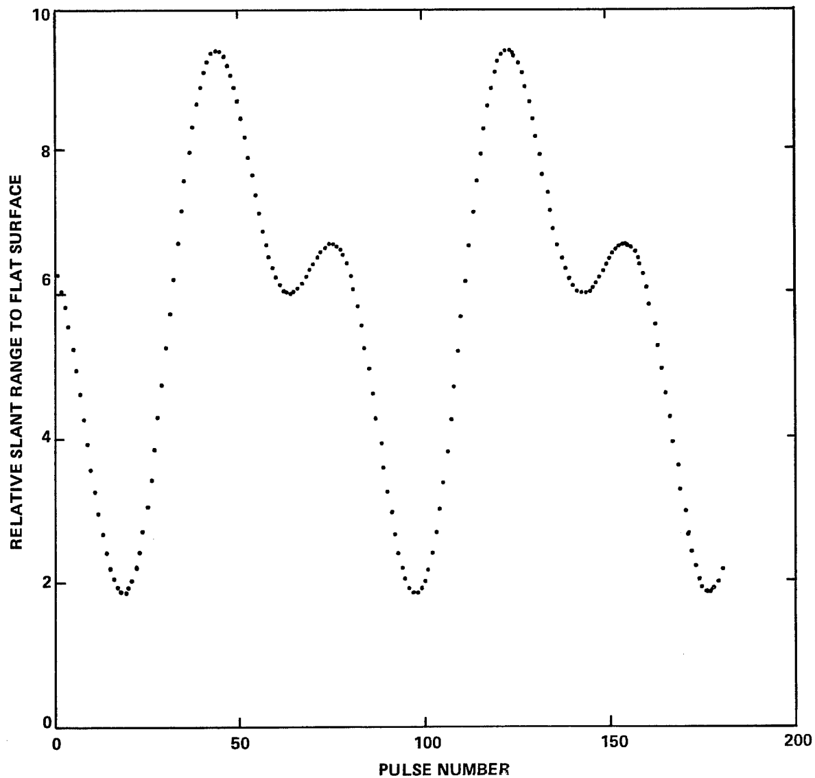
FIGURE 5-35a. AOL SCANNER SLANT ALTITUDE MODEL
