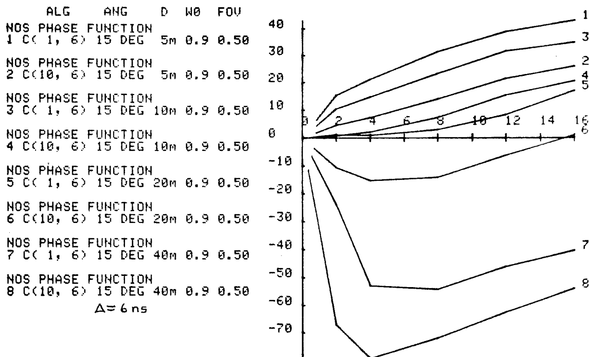
FIGURE 9-30. DEPTH MEASUREMENT BIAS (CM) VS OPTICAL DEPTH
