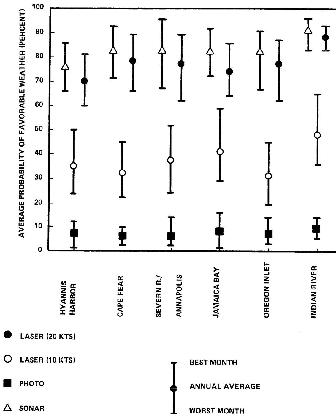
FIGURE 4-4. OCCURRENCE OF FAVORABLE WEATHER
