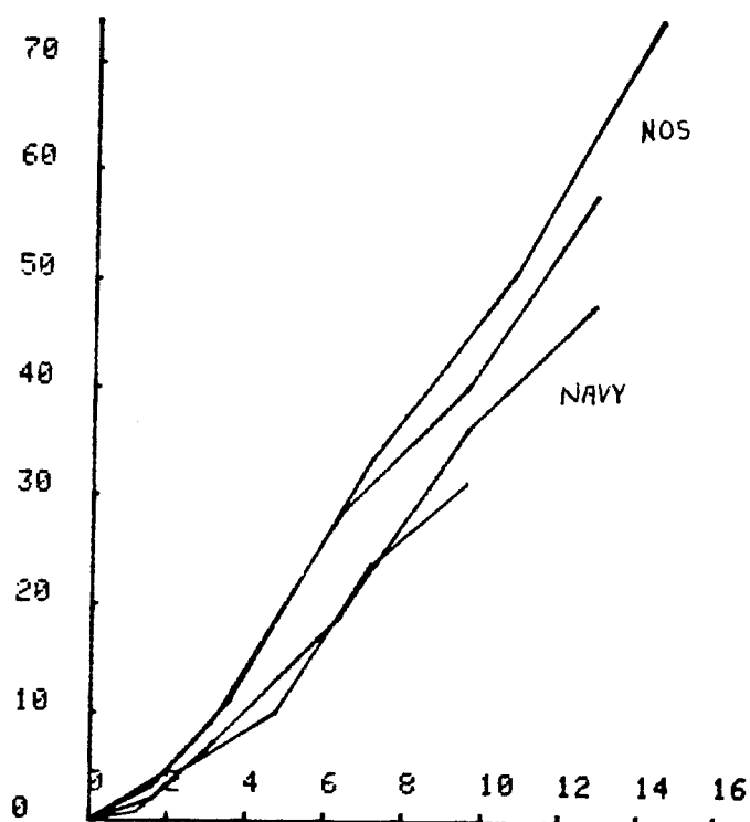
FIGURE 9-19. DEPTH MEASUREMENT BIAS (CM) VS SCATTERING OPTICAL DEPTH
