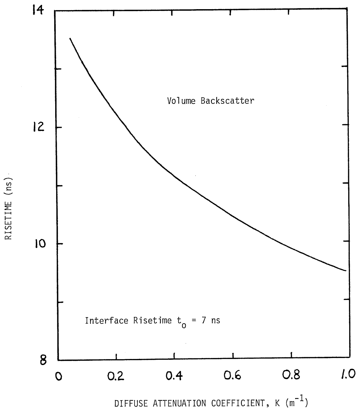
Figure 9-41. Volume Backscatter Risettime (0-100%) vs. K for 7-ns FWHM Triangle Input Pulse
