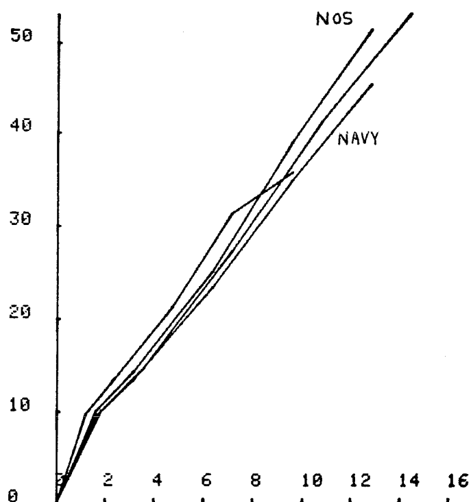
FIGURE 9-20. DEPTH MEASUREMENT BIAS (CM) VS SCATTERING OPTICAL DEPTH
