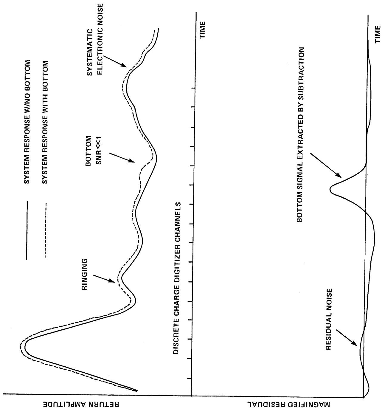
FIGURE 5-14. AOL DEEP WATER "CALIBRATION" PROCEDURE
