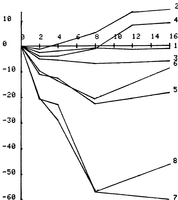
FIGURE 9-28. DEPTH MEASUREMENT BIAS (CM) VS OPTICAL DEPTH
