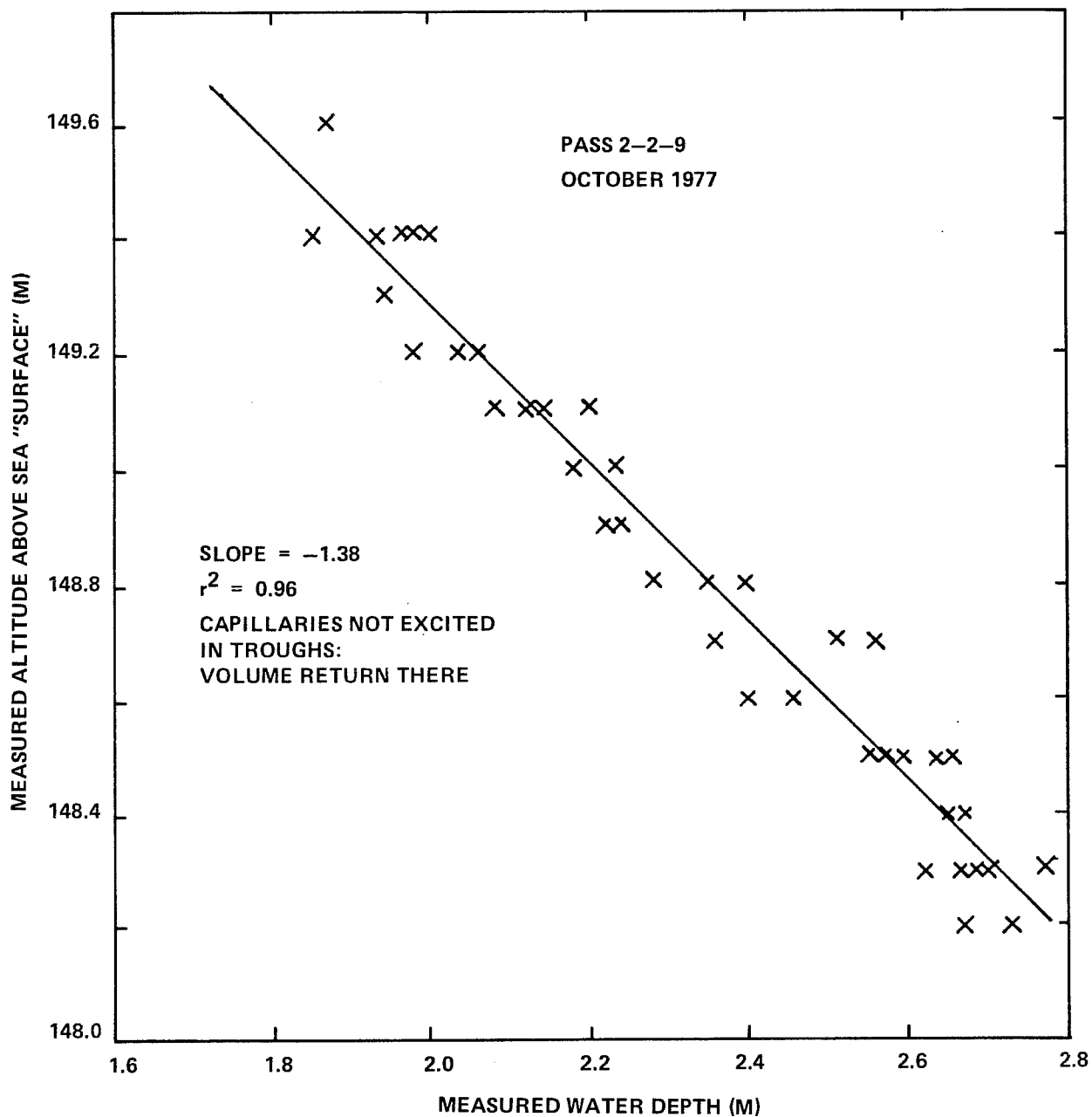
FIGURE 5-33. WAVE CORRELATION IN ALTITUDE AND DEPTH MEASUREMENT
