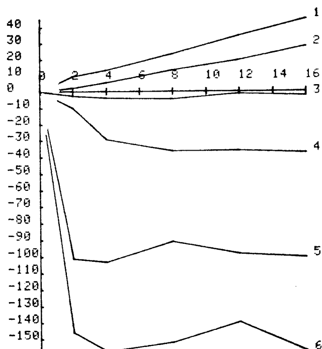
FIGURE 9-15. DEPTH MEASUREMENT BIAS (CM) VS OPTICAL DEPTH
