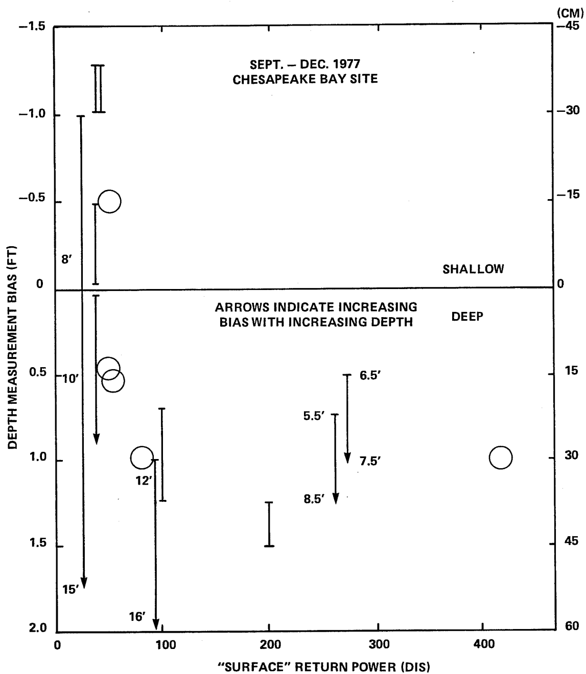
FIGURE 5-44. DEPTH MEASUREMENT BIAS VS. "SURFACE" RETURN POWER
