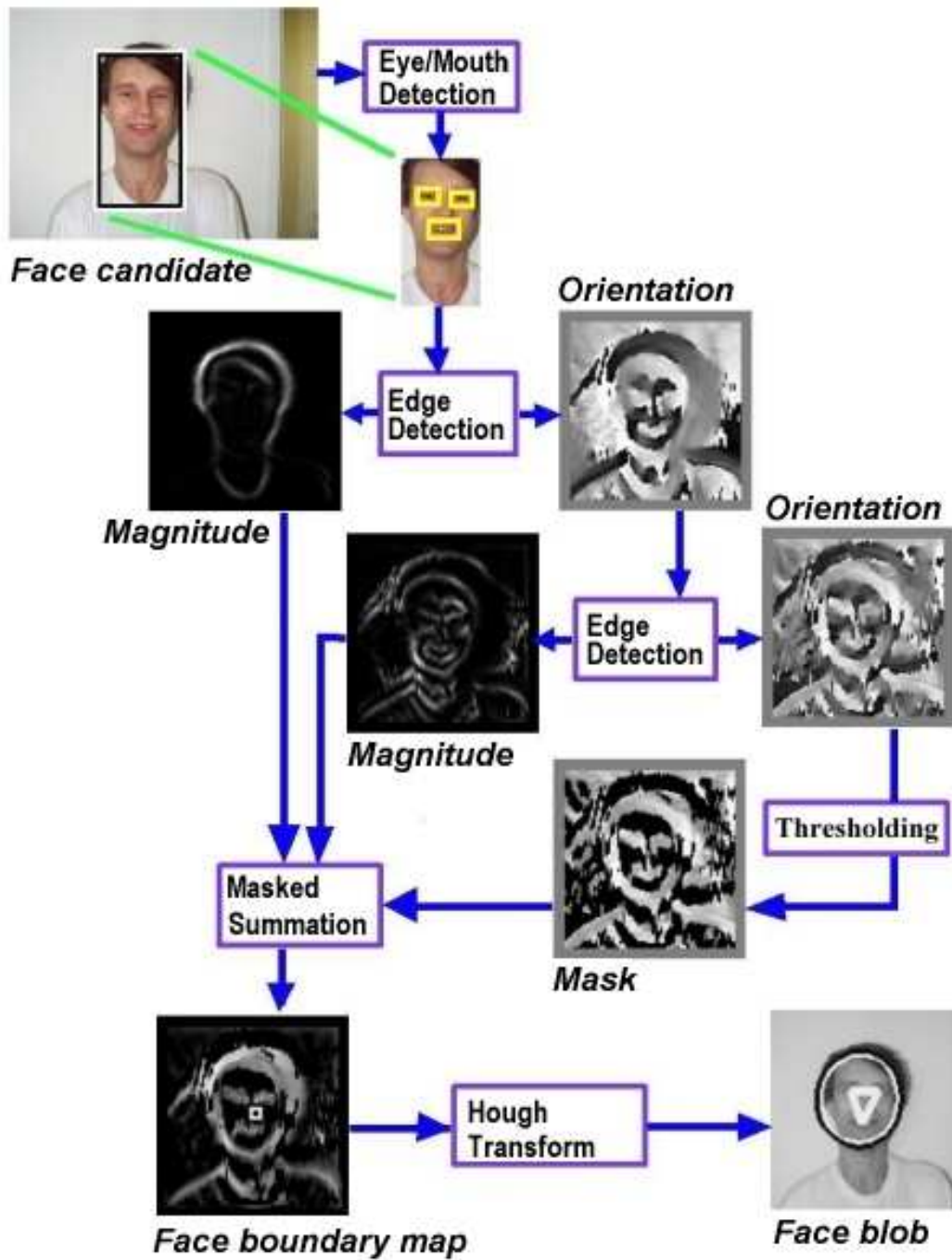
Figure 3.12. Computation of face boundary and the eye-mouth triangle.
