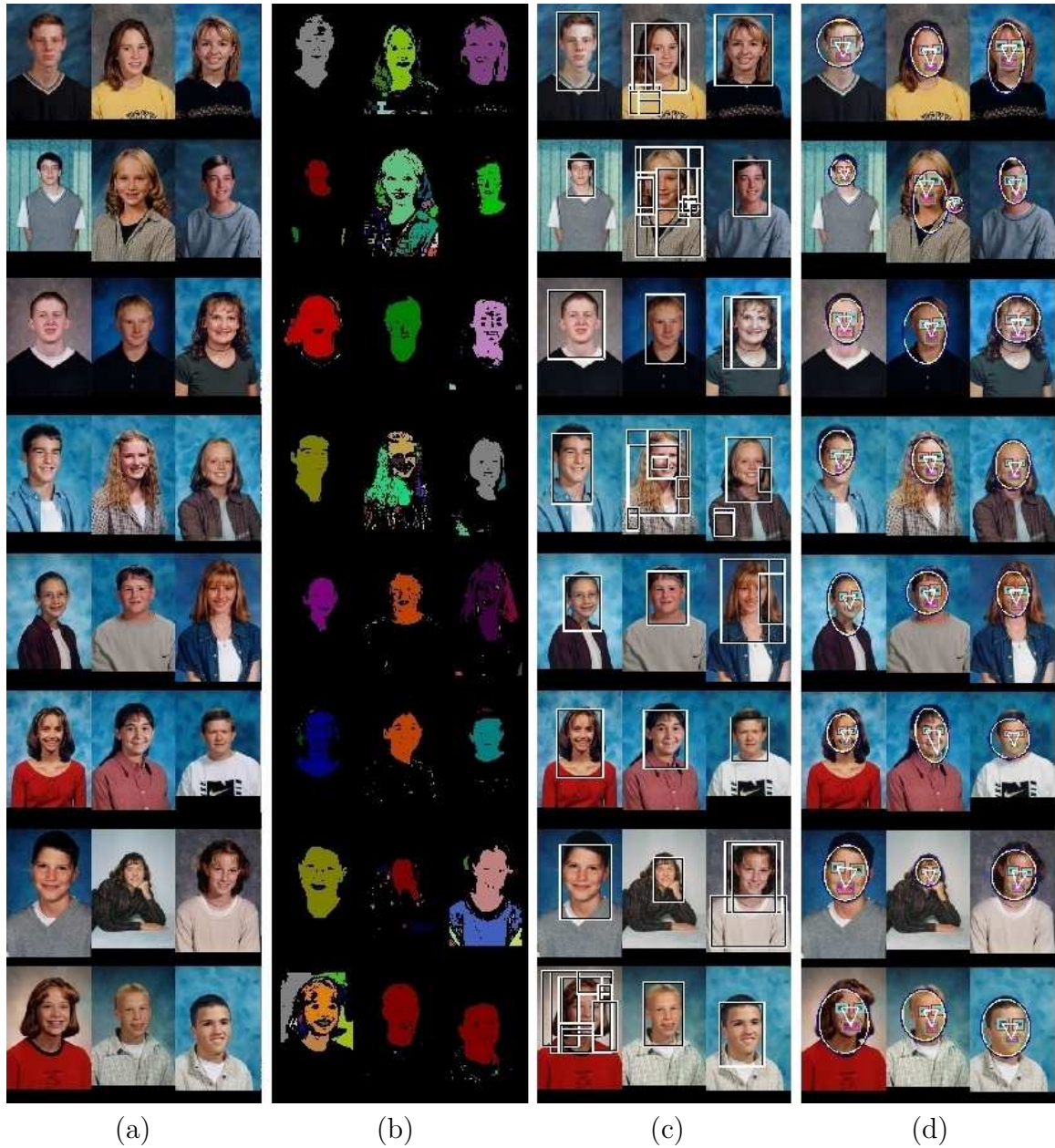
Figure 3.21. Face detection results on a subset of the Champion database: (a) input images; (b) grouped skin regions; (c) face candidates; (d) detected faces are overlaid on the lighting-compensated images.
