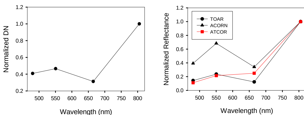
Figure 38. IKONOS vegetation spectral profiles: (left) unprocessed, (right) ATCOR atmospheric correction (shown in red)
