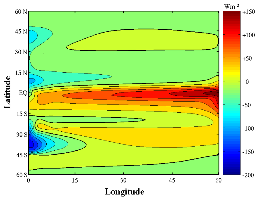
FIGURE 93. As FIGURE 91 except B = -10 (Case P)
