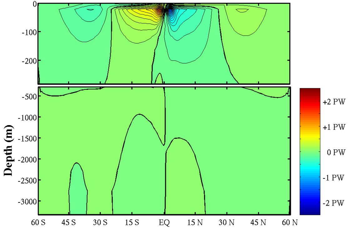
FIGURE 52. Meridional Heat Transport for B = -10 (Case L)
