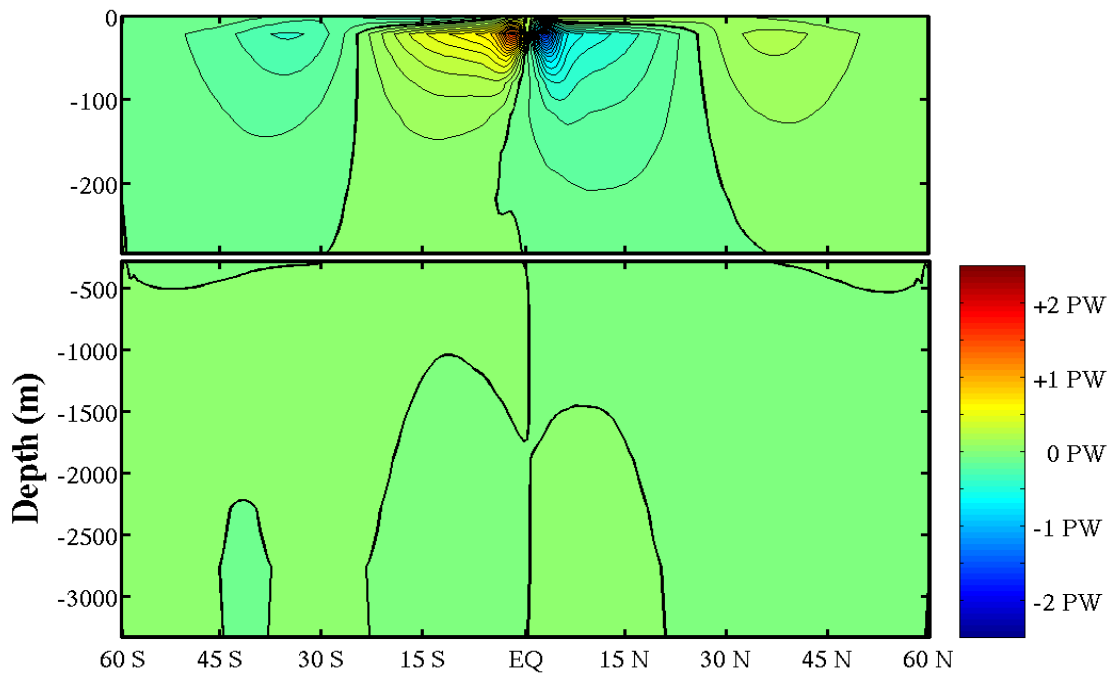
FIGURE 51. Meridional Heat Transport for B = -7.5 (Case K)
