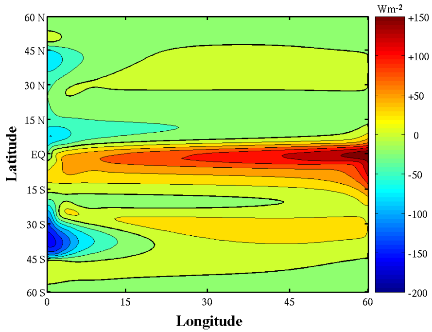
FIGURE 87. As FIGURE 85 except B = -10 (Case G)
