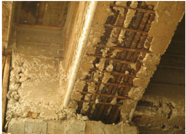
Site Photo 25. Evidence of improperly placed exposed reinforcement bar, PVC conduit, and rust.
