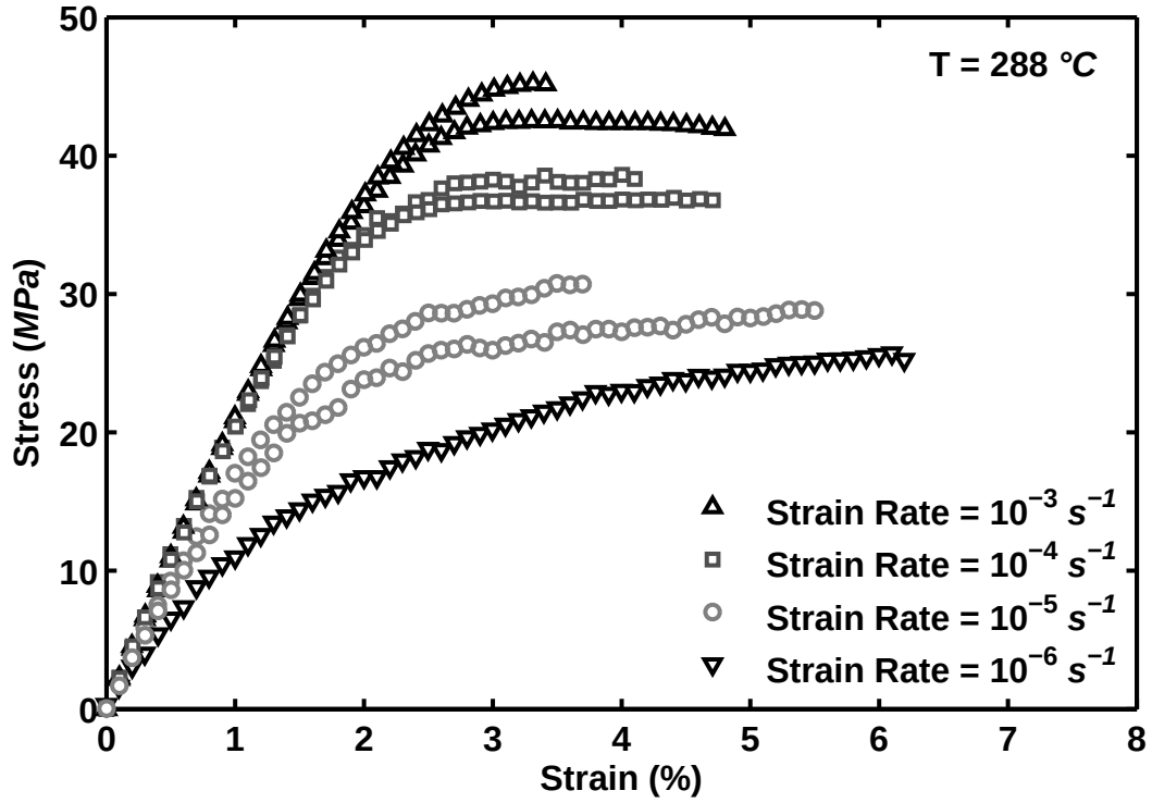
Figure 5.1: Stress-Strain Curves Obtained for PMR-15 in Tensile Test to Failure Conducted at Constant Strain Rates of 10^{-3} , 10^{-4} , 10^{-5} , and 10^{-6} \text{ s}^{-1} at 288^\circ\text{C} . The Dependence of the Stress-Strain Behavior on the Strain Rate is Evident.
