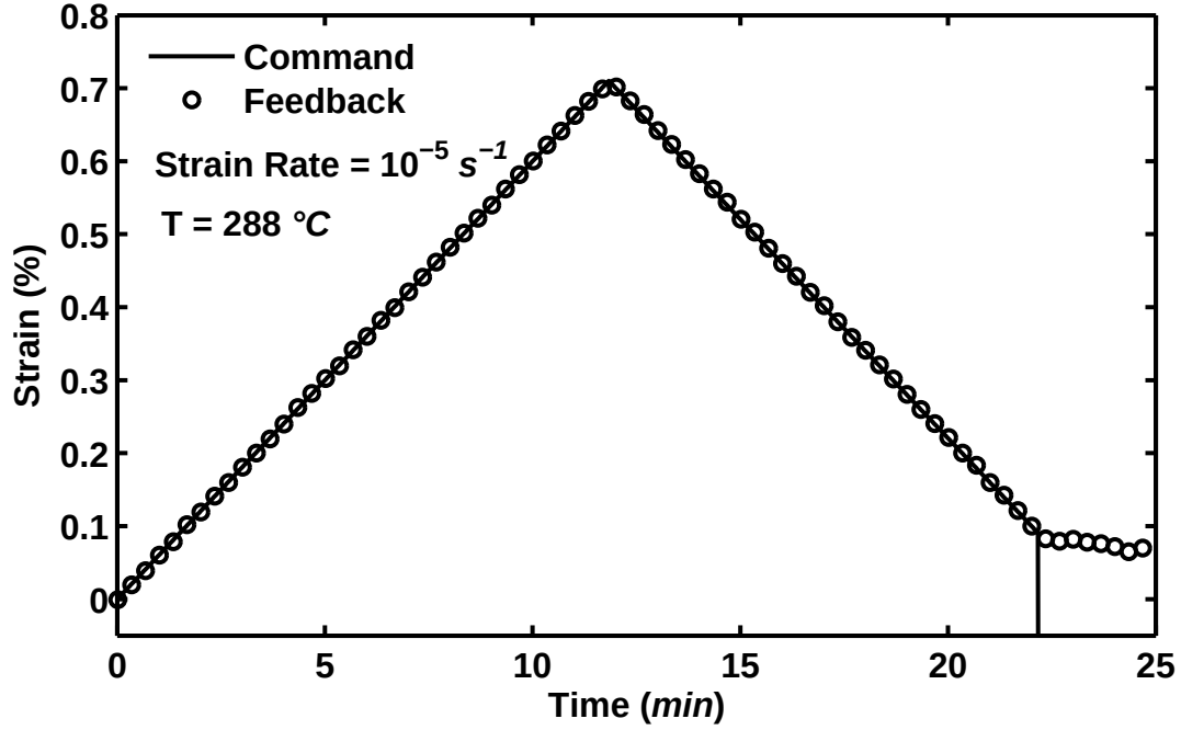
Figure 4.9: Strain Control Tuning with PMR-15 and Low Contact Force Extensometer: Loading and Unloading in Strain Control at 288 \text{ }^{\circ}\text{C} . Strain Rate is 10^{-5} \text{ s}^{-1} .
