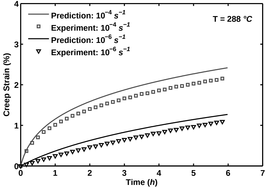
Figure 7.6: Comparison Between the Experimental and Predicted Strain vs Time Curves Obtained for PMR-15 Polymer at 288 \text{ }^{\circ}\text{C} in Creep at 21 \text{ MPa} . Prior Loading at Strain Rates of 10^{-6} and 10^{-4} \text{ s}^{-1} .
