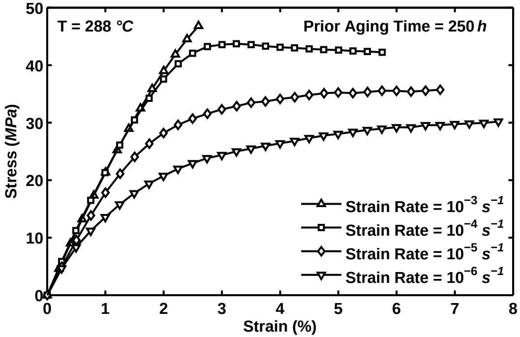
Figure 8.1: Stress-Strain Curves for PMR-15 Specimens Aged for 250 h at 288 ^{\circ}C in Argon Obtained in Tensile Tests to Failure Conducted at Constant Strain Rates of 10^{-6} , 10^{-5} , 10^{-4} , and 10^{-3} s^{-1} at 288 ^{\circ}C . The Dependence of the Stress-Strain Behavior on the Strain Rate is Evident.
