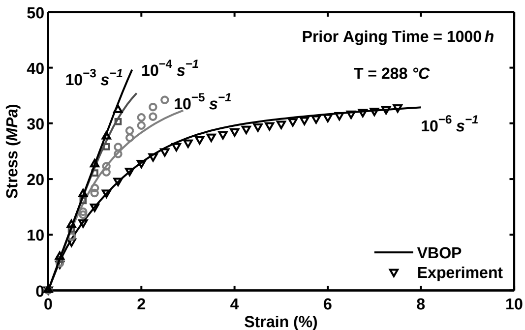
Figure 10.13: A Comparison Between Experimental Results and Simulated Stress-Strain Curves Obtained for PMR-15 Polymer Aged for 1000 h at 288 ^{\circ}C in Argon in Tensile Tests to Failure Conducted at Constant Strain Rates of 10^{-6} , 10^{-5} , 10^{-4} , and 10^{-3} s^{-1} at 288 ^{\circ}C . The Model Successfully Represents the Strain Rate Dependence of the Aged Material.
