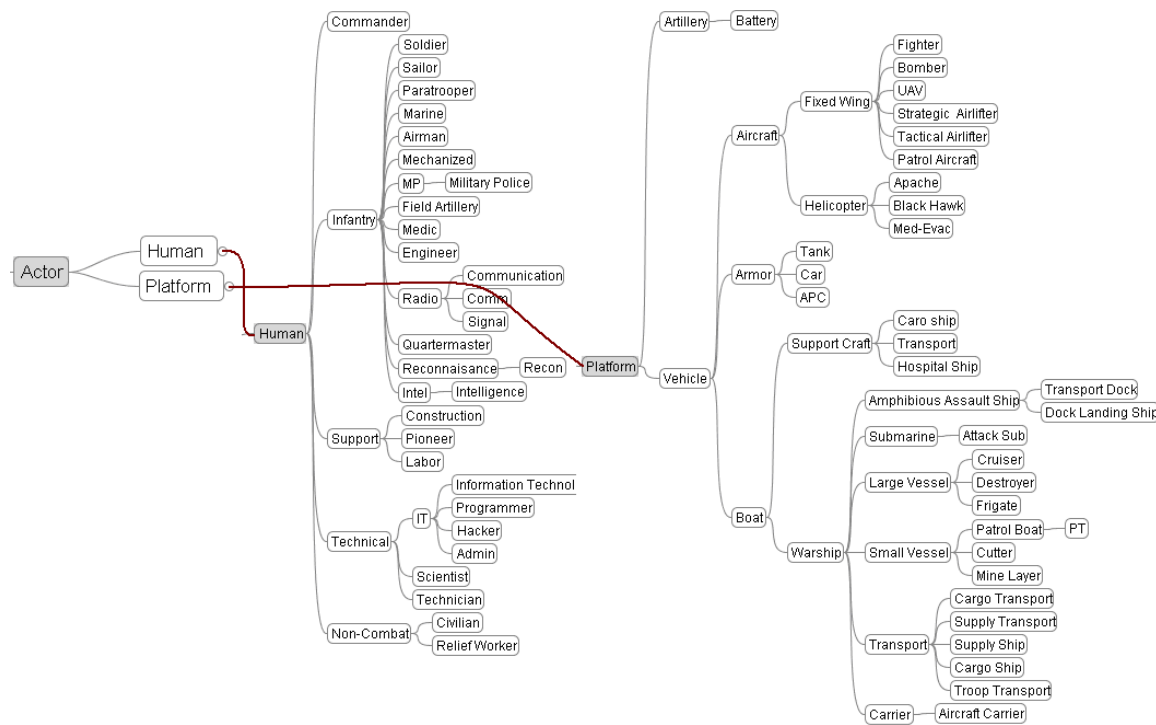
Figure 4 - Actor Taxonomy
