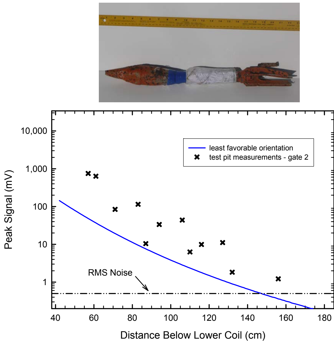
Figure 14 – EM61-MK2 signal at the second time gate as a function of the distance of the center of a 2.36-in Rocket Propelled Grenade below the sensor's bottom coil. The predicted response to the object in its least favorable orientation is shown as a solid line, test pit measurements are plotted as crosses, and the site noise is shown as a dot-dash line.
