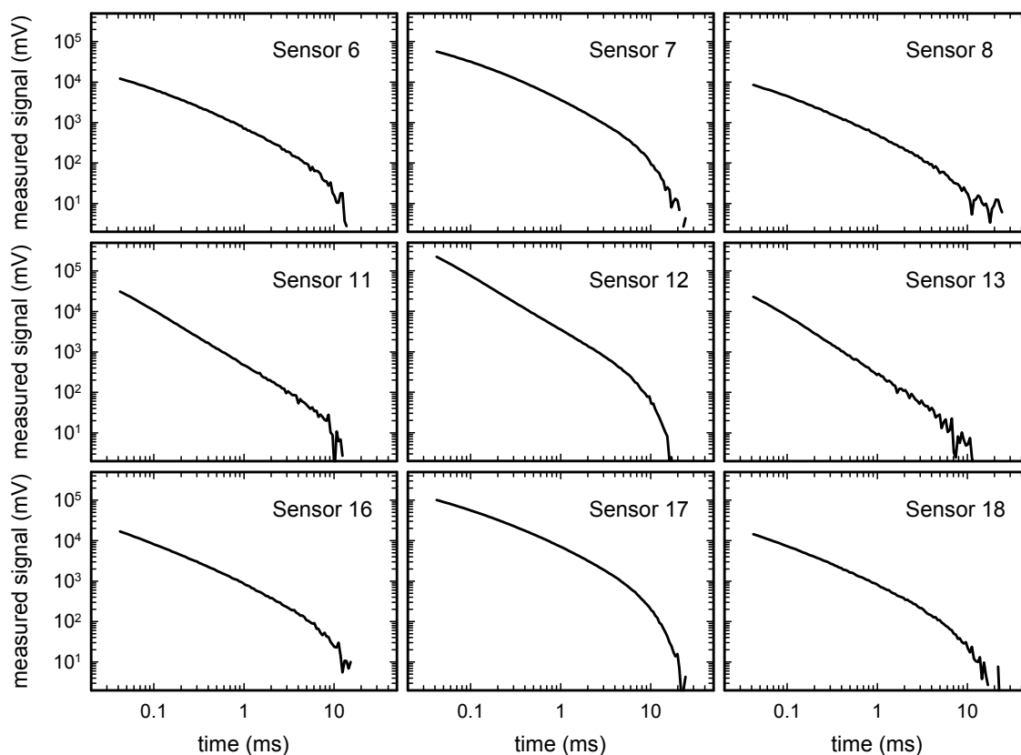
Figure 5 – Measured response of a 2.75-in warhead oriented horizontally along track 35 cm below the TEM array. The nine decays shown represent the response of the nine central receivers (see Figure 3) when the corresponding transmitter is energized.
