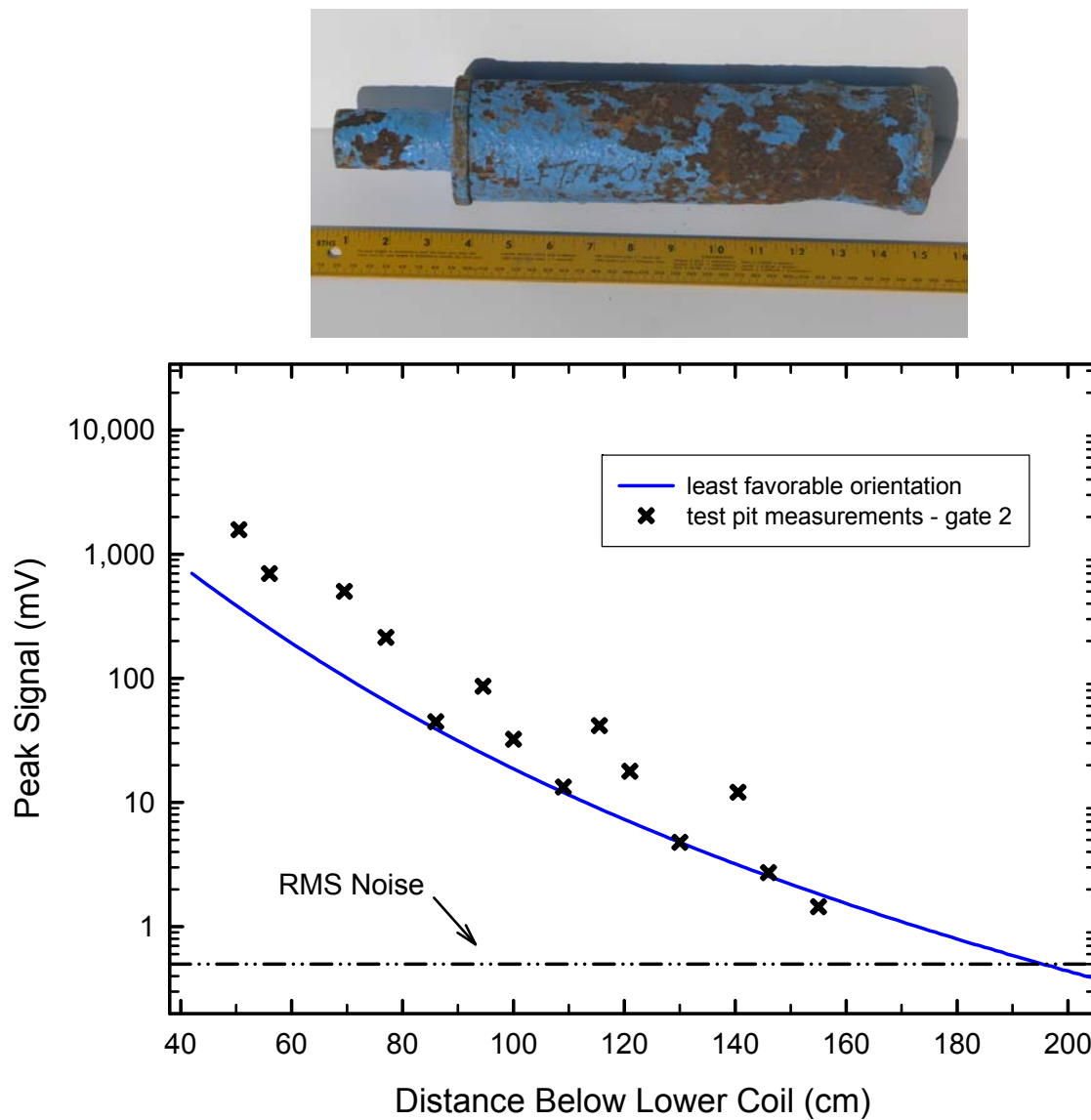
Figure 11 – EM61-MK2 signal at the second time gate as a function of the distance of the center of a 3-in Stokes mortar below the sensor's bottom coil. The predicted response to the object in its least favorable orientation is shown as a solid line, test pit measurements are plotted as crosses, and the site noise is shown as a dot-dash line.
