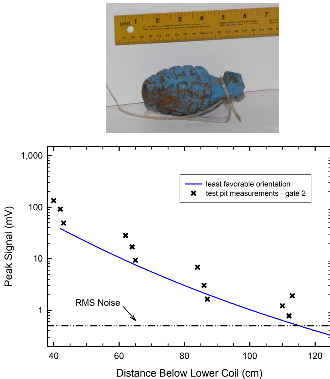
Figure 18 – EM61-MK2 signal at the second time gate as a function of the distance of the center of a hand grenade below the sensor's bottom coil hand grenade. The predicted response to the object in its least favorable orientation is shown as a solid line, test pit measurements are plotted as crosses, and the site noise is shown as a dot-dash line.
