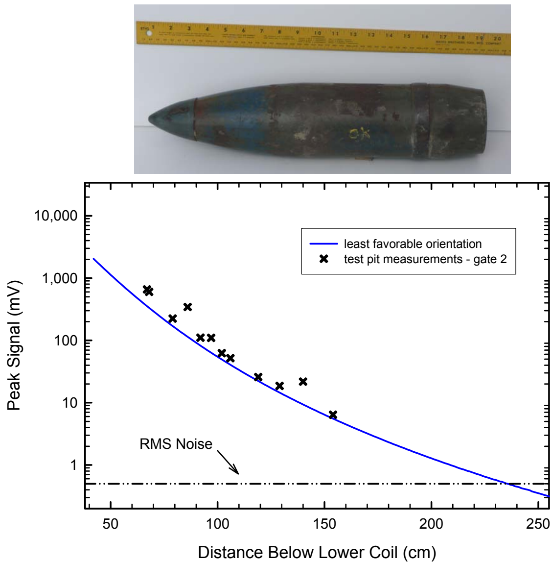
Figure 8 – EM61-MK2 signal at the second time gate as a function of the distance of the center of a 105-mm projectile below the sensor's bottom coil. The predicted response to the object in its least favorable orientation is shown as a solid line, test pit measurements are plotted as crosses, and the site noise is shown as a dot-dash line.
