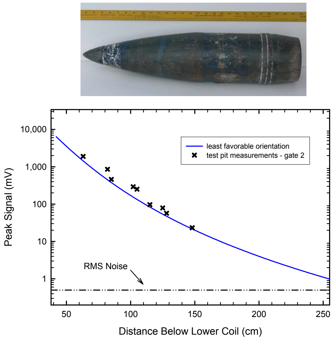
Figure 6 – EM61-MK2 signal at the second time gate as a function of the distance of the center of a 155-mm projectile below the sensor's bottom coil. The predicted response to the object in its least favorable orientation is shown as a solid line, test pit measurements are plotted as crosses, and the site noise is shown as a dot-dash line.
