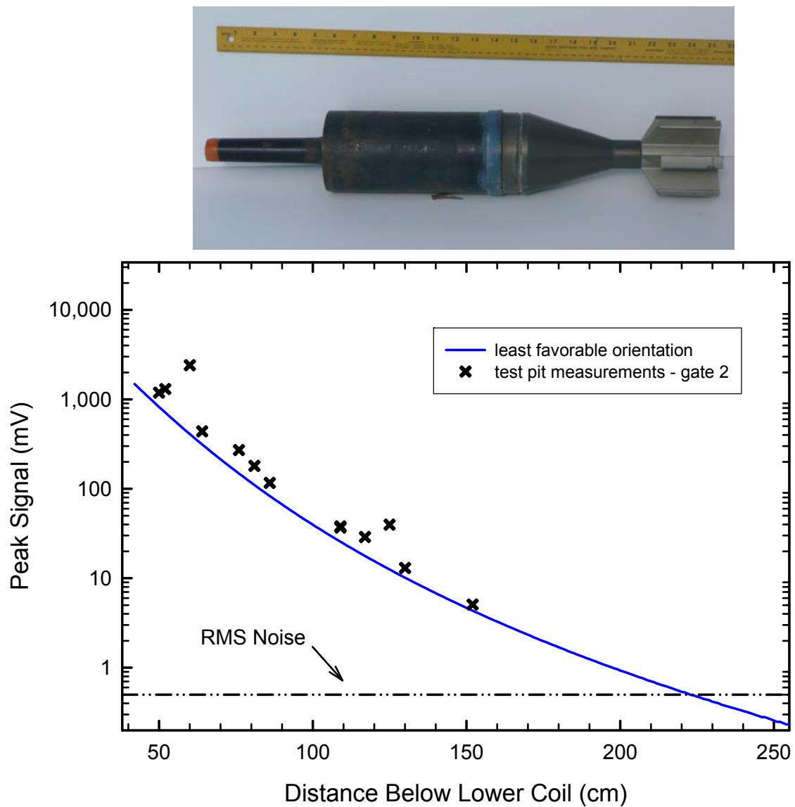
Figure 9 – EM61-MK2 signal at the second time gate as a function of the distance of the center of a 105-mm HEAT projectile below the sensor's bottom coil. The predicted response to the object in its least favorable orientation is shown as a solid line, test pit measurements are plotted as crosses, and the site noise is shown as a dot-dash line.
