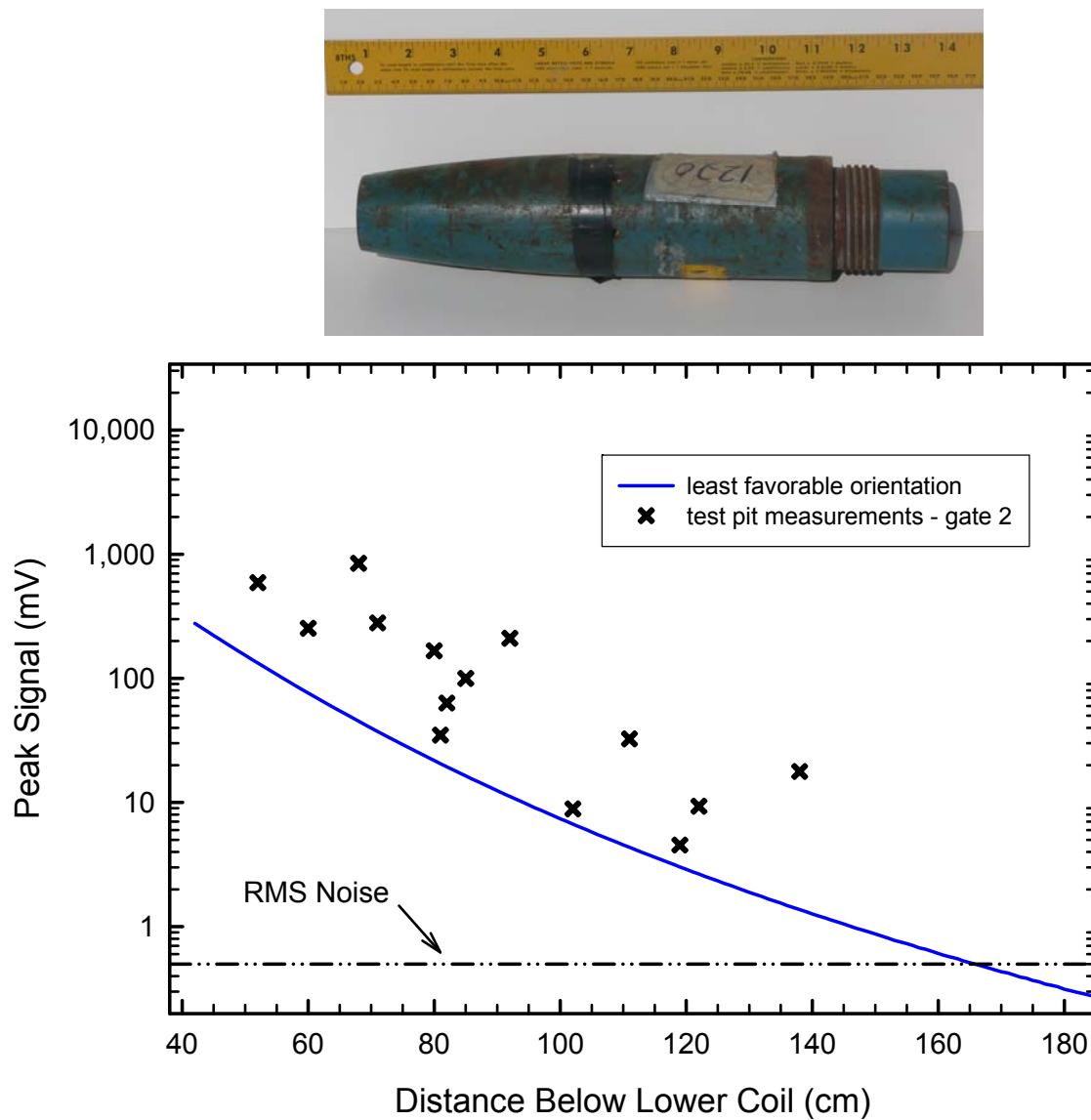
Figure 13 – EM61-MK2 signal at the second time gate as a function of the distance of the center of a 2.75-in rocket warhead below the sensor's bottom coil. The predicted response to the object in its least favorable orientation is shown as a solid line, test pit measurements are plotted as crosses, and the site noise is shown as a dot-dash line.
