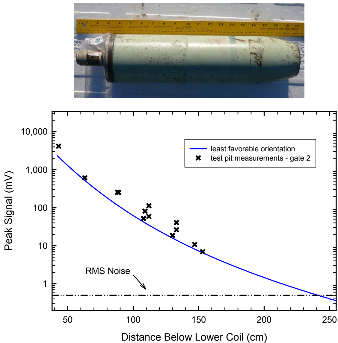
Figure 7 – EM61-MK2 signal at the second time gate as a function of the distance of the center of a 4.2-in mortar below the sensor's bottom coil. The predicted response to the object in its least favorable orientation is shown as a solid line, test pit measurements are plotted as crosses, and the site noise is shown as a dot-dash line.
