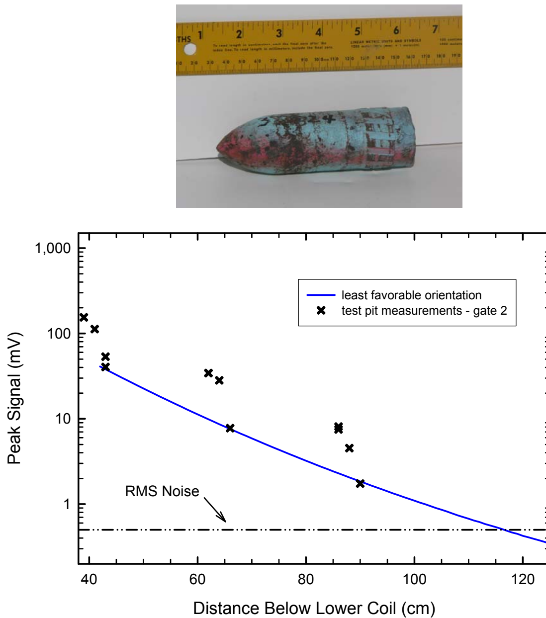
Figure 17 – EM61-MK2 signal at the second time gate as a function of the distance of the center of a 37-mm projectile below the sensor's bottom coil. The predicted response to the object in its least favorable orientation is shown as a solid line, test pit measurements are plotted as crosses, and the site noise is shown as a dot-dash line.
