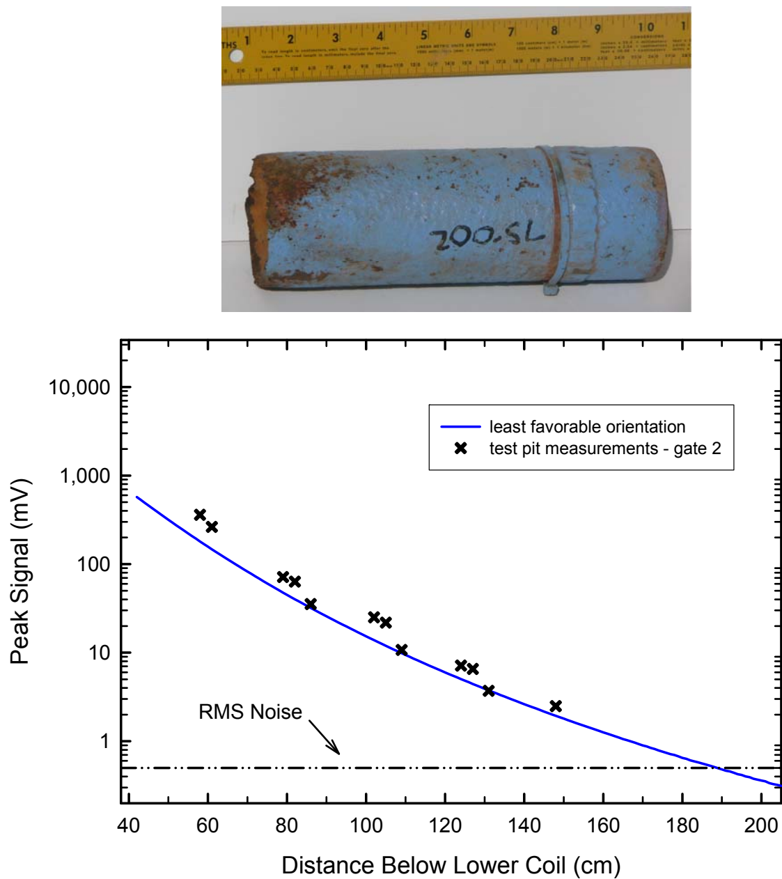
Figure 12 – EM61-MK2 signal at the second time gate as a function of the distance of the center of a 75-mm projectile below the sensor's bottom coil. The predicted response to the object in its least favorable orientation is shown as a solid line, test pit measurements are plotted as crosses, and the site noise is shown as a dot-dash line.
