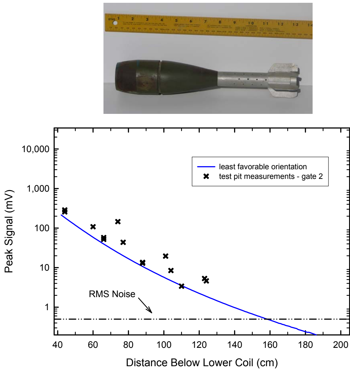
Figure 15 – EM61-MK2 signal at the second time gate as a function of the distance of the center of a 60-mm mortar below the sensor's bottom coil. The predicted response to the object in its least favorable orientation is shown as a solid line, test pit measurements are plotted as crosses, and the site noise is shown as a dot-dash line.
