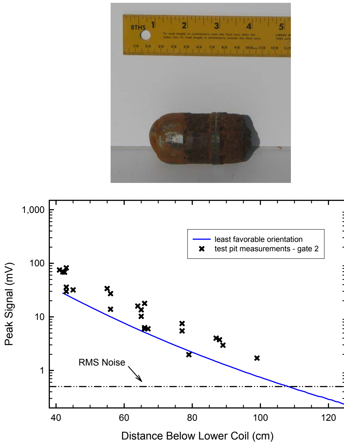
Figure 16 – EM61-MK2 signal at the second time gate as a function of the distance of the center of a 40-mm grenade below the sensor's bottom coil. The predicted response to the object in its least favorable orientation is shown as a solid line, test pit measurements are plotted as crosses, and the site noise is shown as a dot-dash line.
