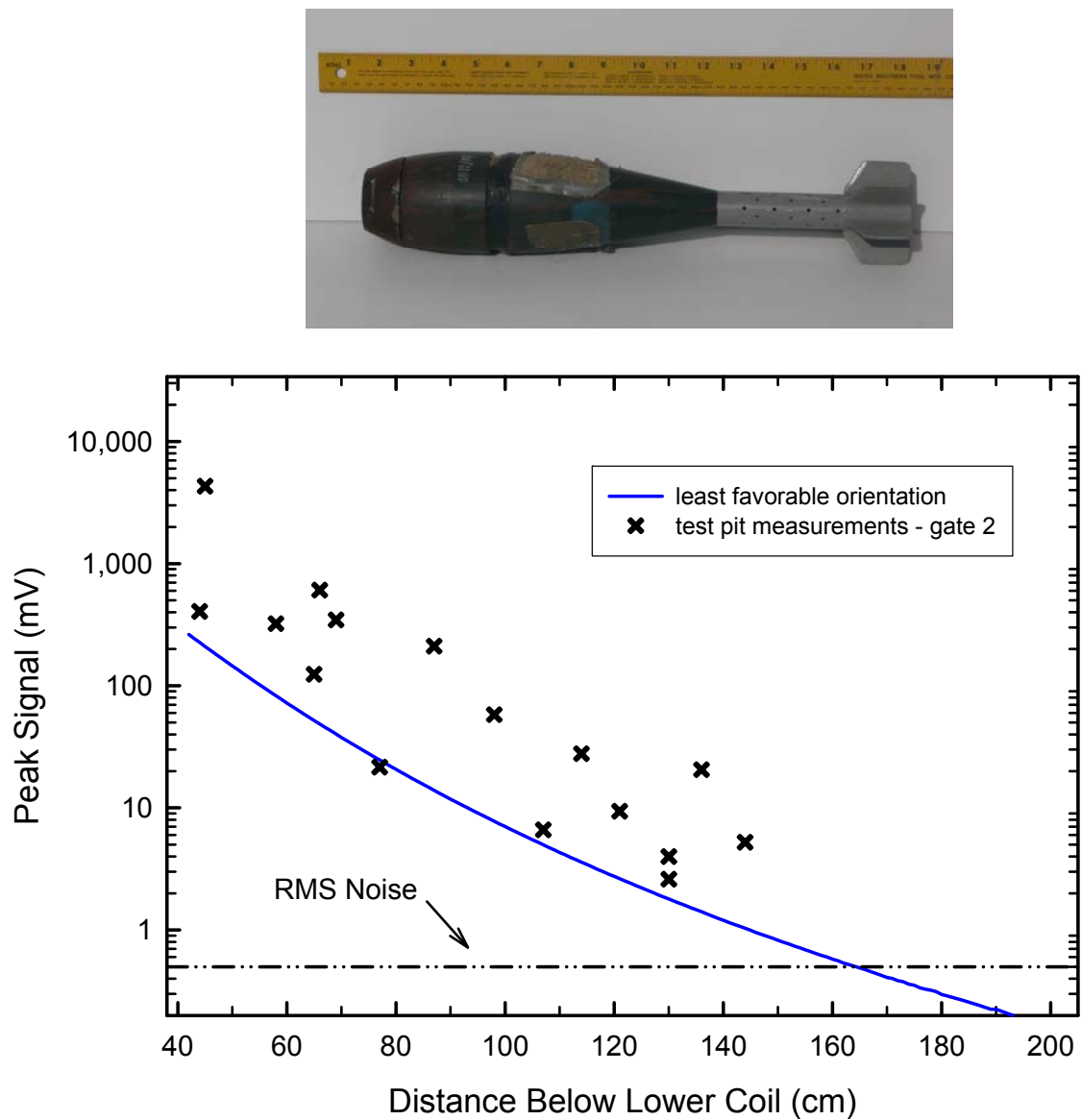
Figure 10 – EM61-MK2 signal at the second time gate as a function of the distance of the center of an 81-mm mortar below the sensor's bottom coil. The predicted response to the object in its least favorable orientation is shown as a solid line, test pit measurements are plotted as crosses, and the site noise is shown as a dot-dash line.
