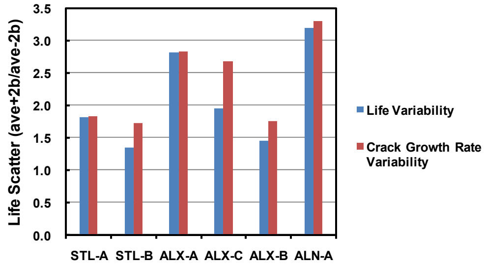
Figure 4: Comparison of the average crack growth rate variability and life variability for the six materials and test conditions (ave is the average life and b is standard deviation of that life distribution).
