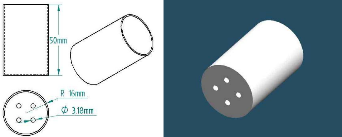
Figure 4: The cylindrical part produced by the injection mold and inserts during experimentation.
