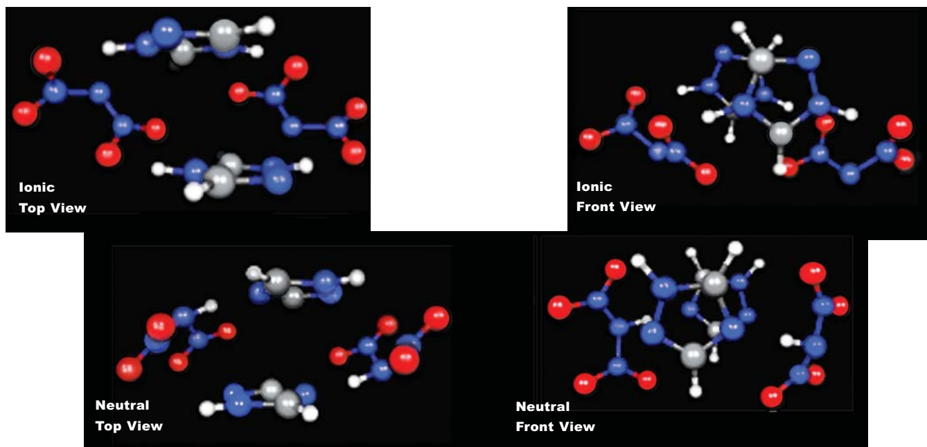
Figure 1. MP2/aug-cc-pVDZ optimized structures of two pairs of 1,2,4-triazolium (1,2,4-triazole) and dinitramide (dinitramine) molecules. H is white, C is gray, O is red, N is blue.
