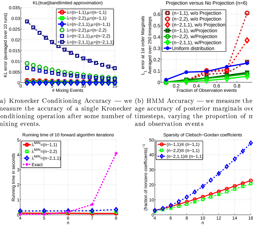
(c) Running times: We compared running times of our polynomial time bandlimited inference algorithms against an exact algorithm with O(n^3 n!) time complexity. (d) Clebsch-Gordan Sparsity: We measured the sparsity of the Clebsch-Gordan coefficients matrices by plotting the reciprocal of the fraction of nonzero entries against n . A straight line in the plot means that the number of nonzero entries scales linearly in n , and a convex curve scales better than linearly.
