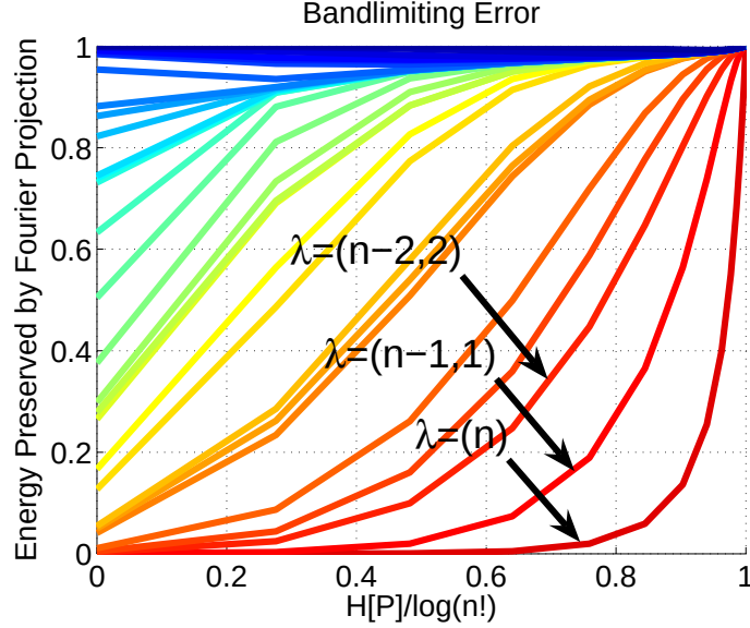
Figure 5: In general, smoother distributions are well approximated by low-order Fourier projections. In this graph, we show the approximation quality of the Fourier projections on distributions with different entropies, starting from sharply peaked delta distributions on the left side of the graph, which get iteratively smoothed until they become the maximum entropy uniform distribution on the right side. On the y -axis, we measure how much energy is preserved in the bandlimited approximation, which we define to be \frac{|P'|^2}{|P|^2} , where P' is the bandlimited approximation to P . Each line represents the approximation quality using a fixed number of Fourier coefficients. At one extreme, we achieve perfect signal reconstruction by using all Fourier coefficients, and at the other, we perform poorly on “spiky” distributions, but well on high-entropy distributions, by storing a single Fourier coefficient.
