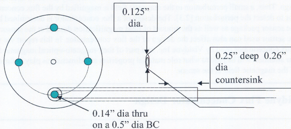
Figure 2. Bolt hole configuration in end caps of permalloy concentrators.
