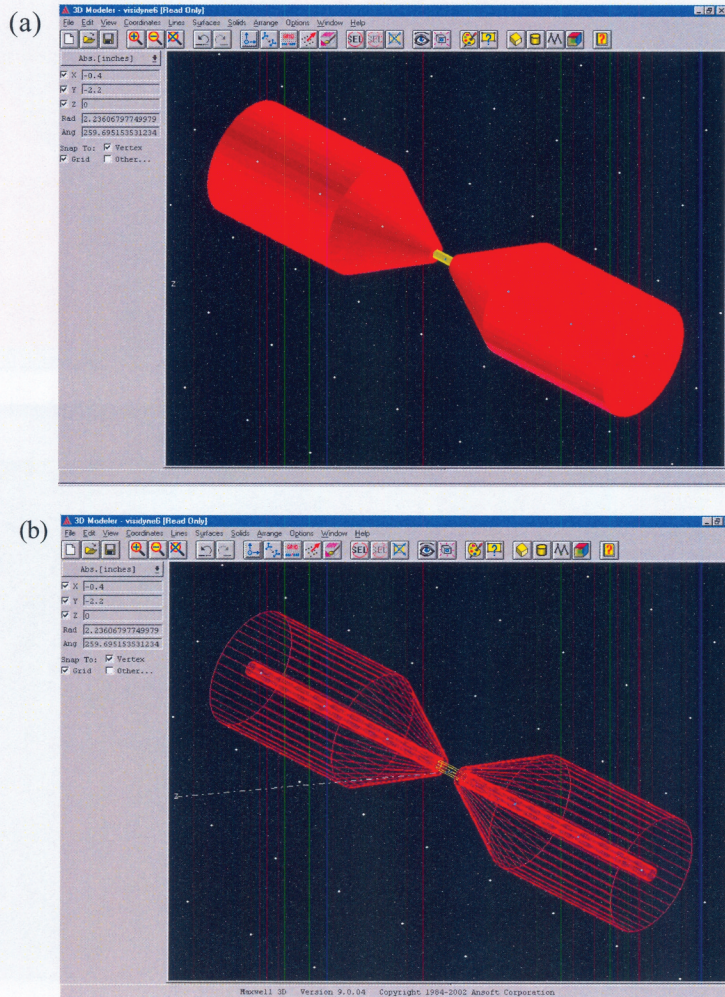
Figure 3. Three dimensional drawing of flux concentrator, (a) shaded and (b) wire frame. The red objects are permalloy, the yellow is the YIG crystal.
