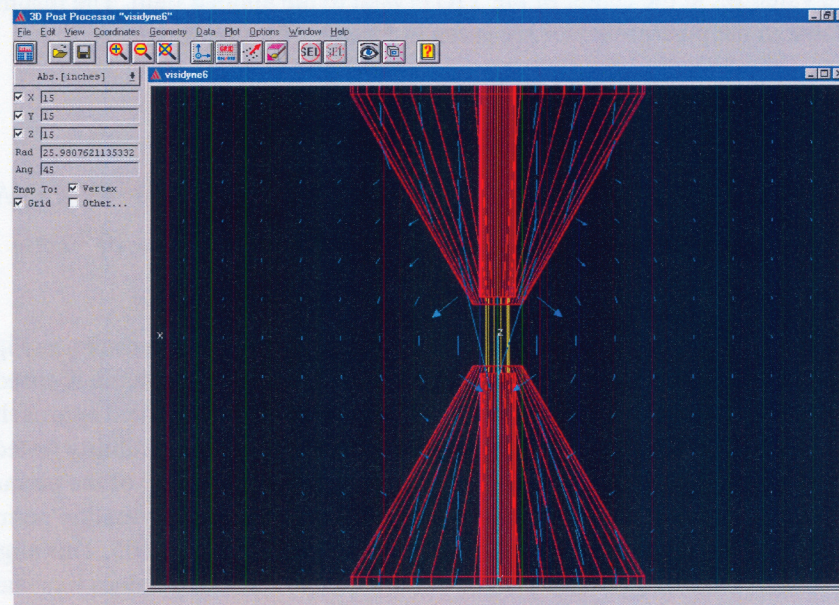
Figure 6. Plot of the magnetic flux density B in the x - y plane, looking down the z -axis.
