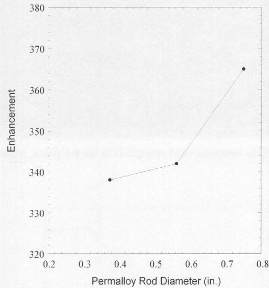
Figure 9. Plot of changes in enhancement factor as diameter of permalloy rod is changed.
