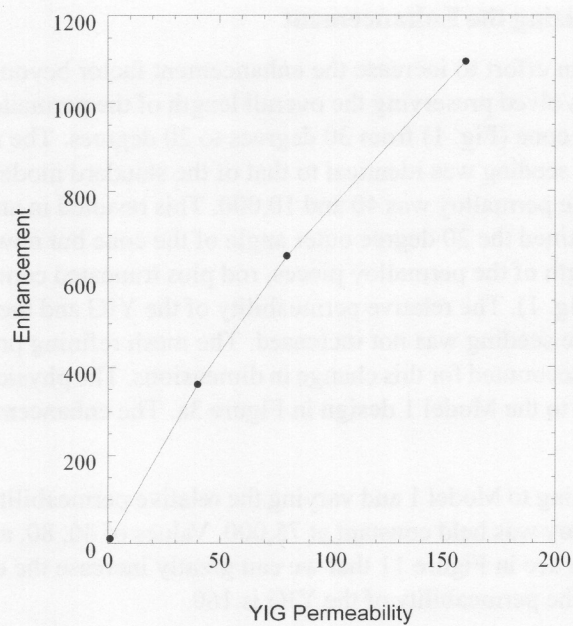
Figure 11. Plot of changes in enhancement as the relative permeability of the YIG crystal is increased. Permeability of the permalloy is held constant at 75,000.
