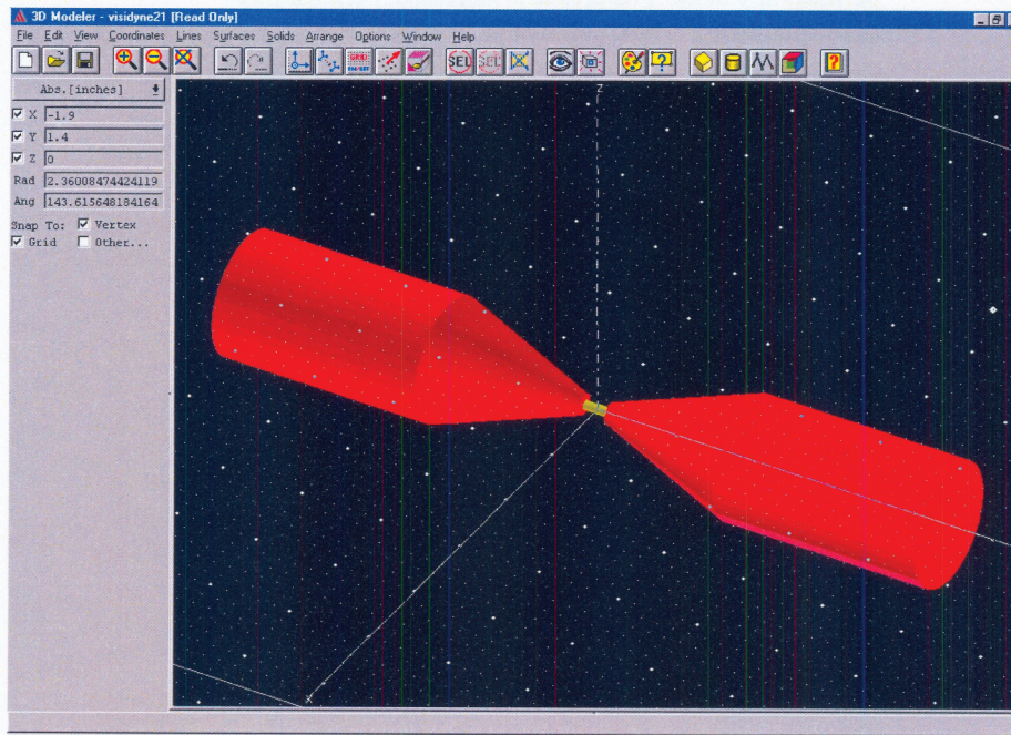
Figure 10. Physical design of flux concentrator incorporating changes of rod length and truncated cone angle.
