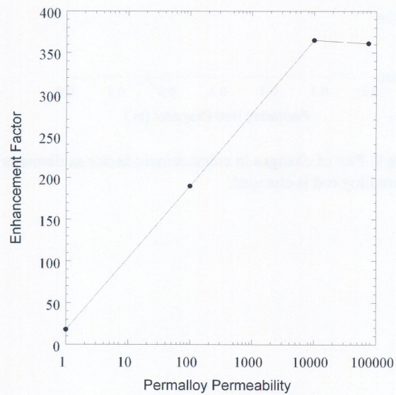
Figure 8. Plot of changes in enhancement factor as the permalloy permeability changed. Please note the x-axis is log scale. YIG permeability held constant at 40.
