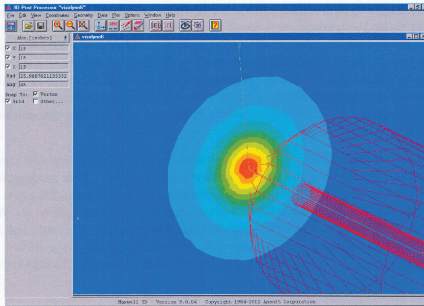
Figure 5. Plot of H in the x - z plane, through the origin. Progression from blue to red indicates increasing field strengths from the background to the center of the YIG.
