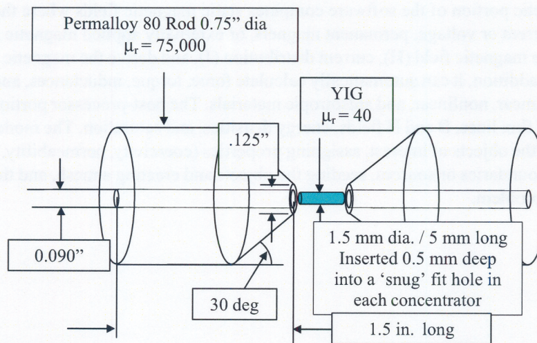
Figure 1. The Visidyne flux concentrator design.
