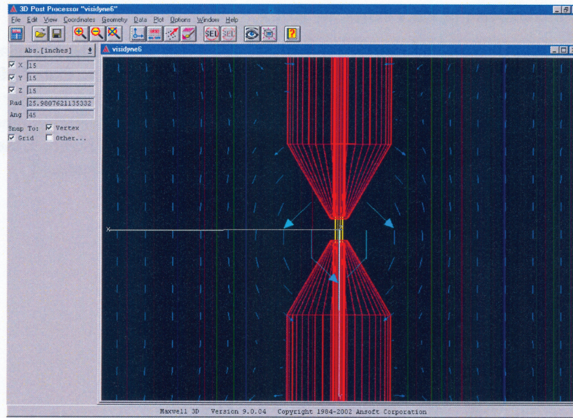
Figure 7. Plot of the magnetic field strength H in the x-y plane, looking down the z-axis.
