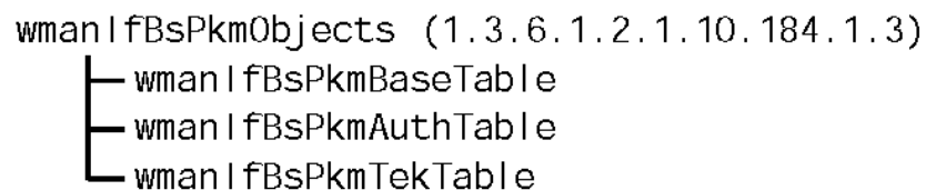
Figure 12. wmanIfBsPdmObjects Structure
