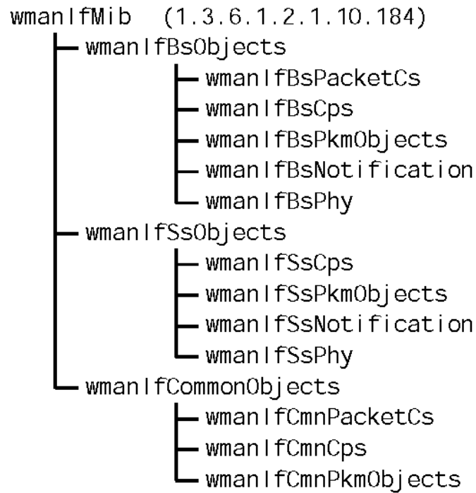
Figure 9. wmanIfMib Structure
