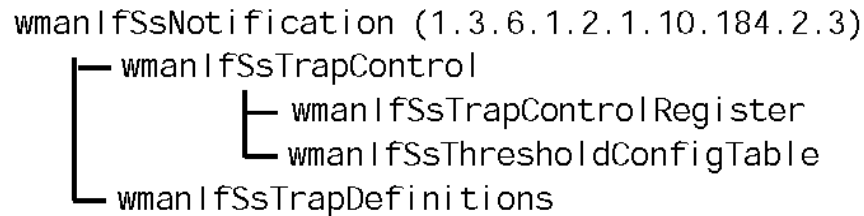
Figure 18. wmanIfSsNotification Structure
