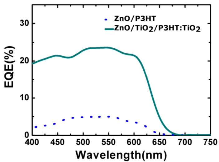
Fig.4 (a) Photovoltaic performances of the devices based on the ZnO/P3HT and ZnO/TiO 2 nanorods /P3HT:TiO 2 nanorods hybrid under simulated AM 1.5 illumination ( 100 \text{ mW}/\text{cm}^2 ). (b) External quantum efficiency (EQE) as a function of wavelength.
