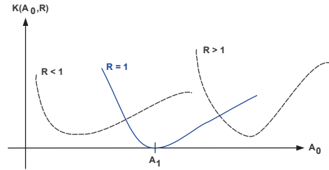
Fig. 3. The error exponent K(A_0, R) versus A_0 for fixed A_1 and R = 1 , R > 1 , and R < 1 . Note that f_0(R) = \arg \min_{A_0} K(A_0, R) is increasing in R , and f_0(1) = A_1 .
