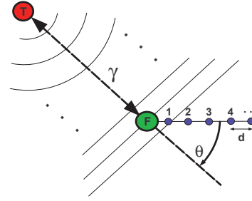
Fig. 2. System model. Each sensor (1, \dots, N) takes a sample of the signal field. Samples are collected on a straight line with spacing d and delivered to the fusion center F . The sensor network is in the far-field of the target T at a relative distance \gamma , and contours of the signal intersect the collection line at an angle \pi/2 - \theta .
