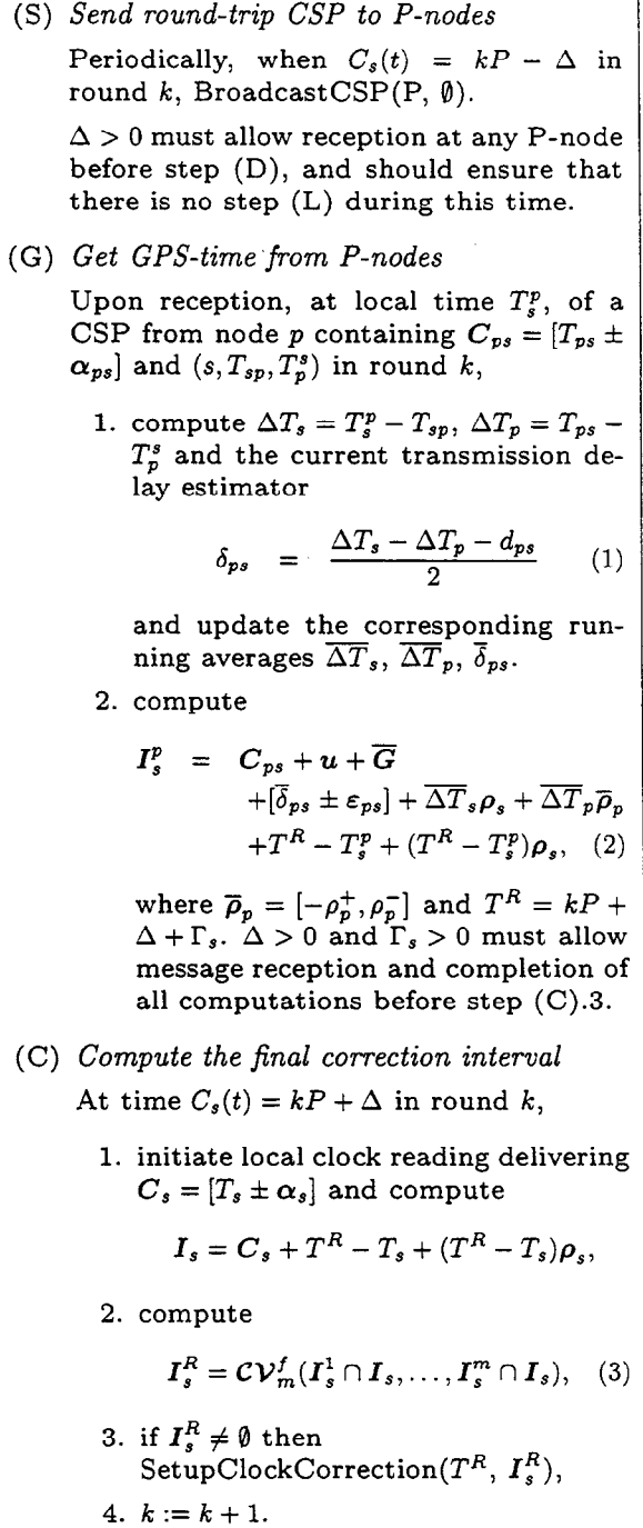
Figure 9: Time distribution algorithm: S-nodes
