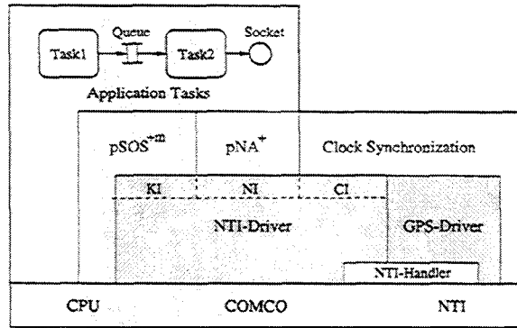
Figure 6: Architecture of a pSOS^{+m} node using the NTI- and GPS-Driver
