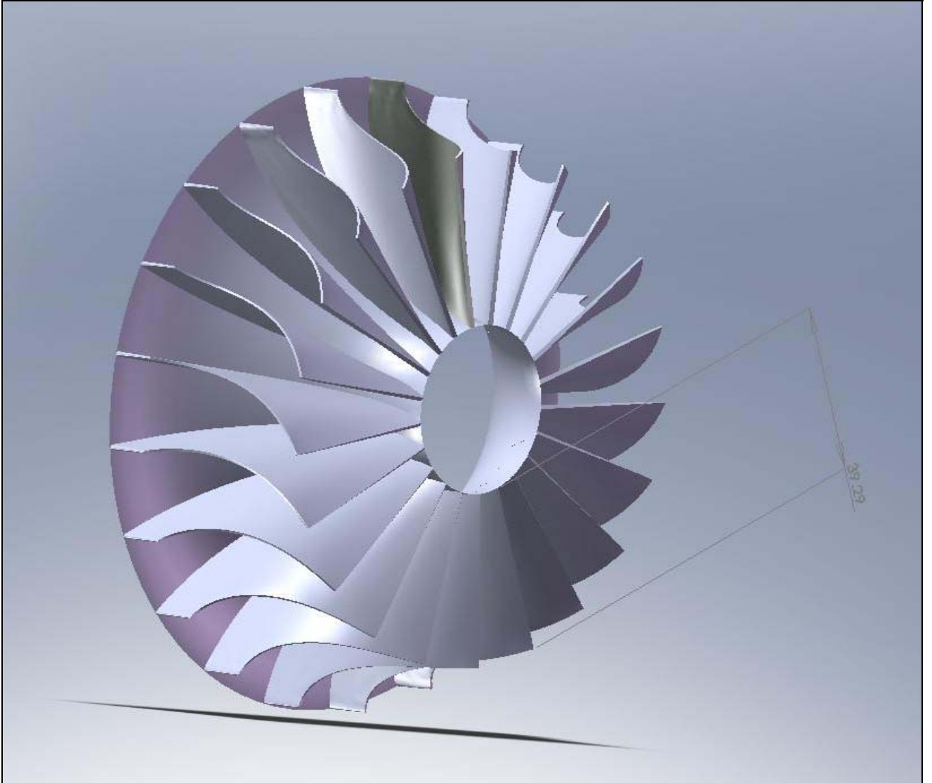
Figure 15: Turbine rotor
