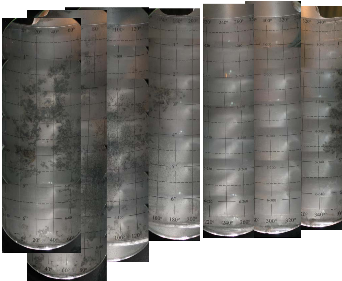
Figure B-3: Photo Montage of Corrosion on Inside Damper Region of Shank 0491
