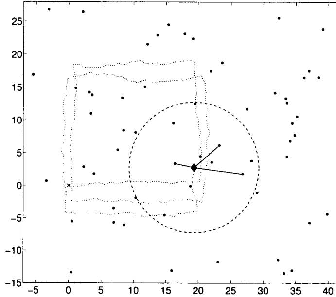
Figure 3-1: A plot of the LG simulation environment. The robot (denoted by the diamond marker) begins at the origin and travels in a series of counterclockwise loops within an environment that consists of 60 point features. The vehicle measures the relative position of a limited number of features that lie within the sensor's FOV, as indicated by the circle.
