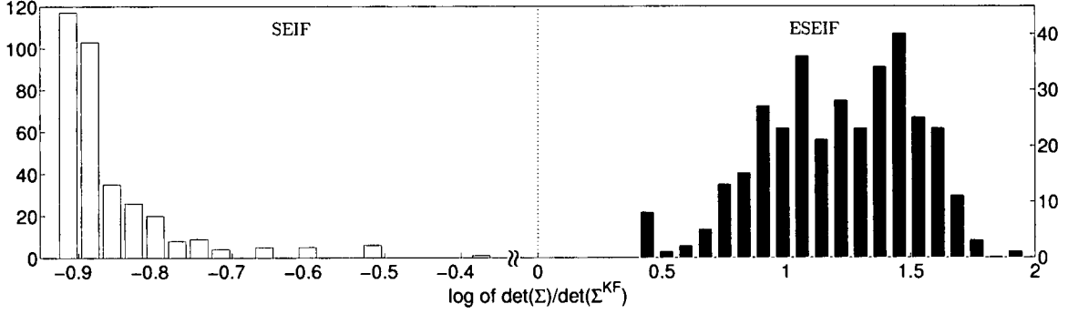
Figure 4-5: Histogram for the LG simulation describing the global map uncertainty maintained by the SEIF ( left ) and ESEIF ( right ) as compared with that of the KF. For each feature, we compute the log of the ratio between the information filter covariance sub-block determinant and the determinant for the actual distribution as given by the KF. Values greater than zero imply conservative estimates for the uncertainty while log ratios less than zero indicate overconfidence. Note that all of the SEIF estimates are overconfident while those of the ESEIF are conservative.
