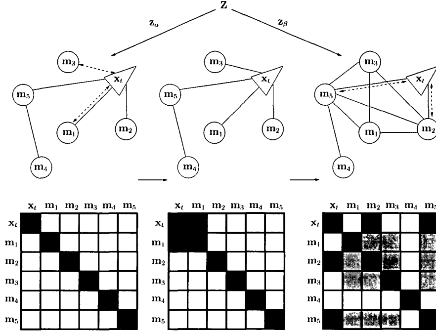
Figure 4-2: A graphical description of the ESEIF sparsification strategy. At time t , the map is comprised of three active features, \mathbf{m}^+ = \{\mathbf{m}_1, \mathbf{m}_2, \mathbf{m}_5\} , and two passive features, \mathbf{m}^- = \{\mathbf{m}_3, \mathbf{m}_4\} , as indicated by the shaded off-diagonal elements in the information matrix. The robot makes three observations of active landmarks, \{\mathbf{z}_1, \mathbf{z}_2, \mathbf{z}_5\} , and one of a passive feature, \mathbf{z}_3 . In the first step of the sparsification algorithm, shown in the left-most diagram, the ESEIF updates the distribution based upon a subset of the measurements, \mathbf{z}_\alpha = \{\mathbf{z}_1, \mathbf{z}_3\} . The result is a stronger constraint between \mathbf{m}_1 and the robot, as well as the creation of a link with \mathbf{m}_3 , which we depict in the middle figure. Subsequently, the ESEIF marginalizes out the vehicle pose, leading to connectivity among the active landmarks. The schematic on the right demonstrates the final step of sparsification in which the robot is relocated within the map based upon the remaining \mathbf{z}_\beta = \{\mathbf{z}_2, \mathbf{z}_5\} measurements. The result is a joint posterior, p_{\text{ESEIF}}(\xi_t | \mathbf{z}^t, \mathbf{u}^t) , represented by an exactly sparse information matrix where the size of the active map is controlled.
