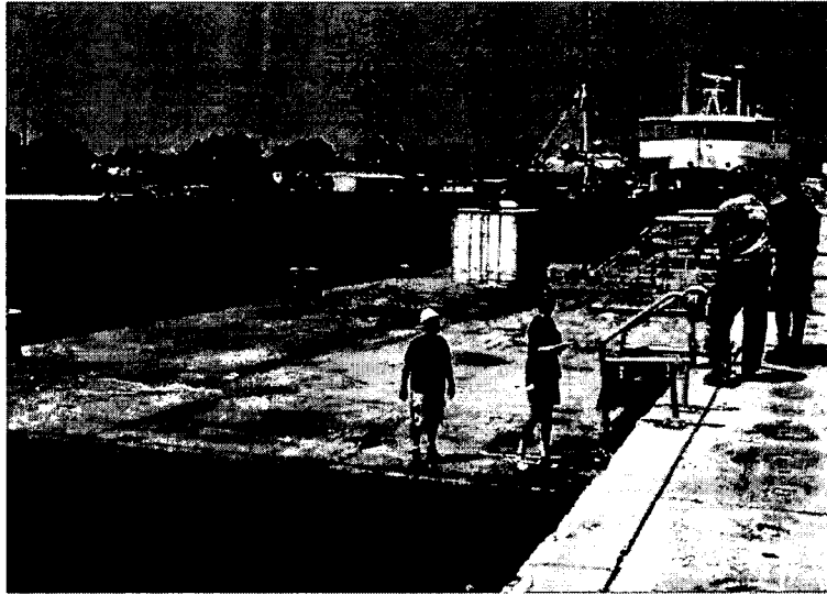
Figure 5-6: The first version of the HAUV being lowered into the water to survey the barge during AUVFest. The barge is 13.4 m from port (side nearest to the pier) to starboard and 36.2 m from bow to stern.
