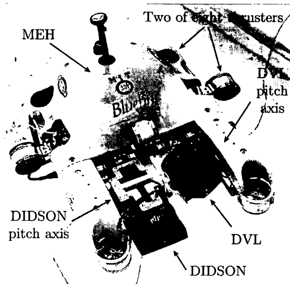
Figure 5-1: Version 1B of the HAUV. The vehicle is roughly 90 cm ( L ) \times 85 cm ( W ) \times 44 cm ( H ) in overall size and weighs approximately 90 kg. Eight ductless thrusters provide for full maneuverability. At the front of the vehicle are the DIDSON imaging sonar and DVL that can be independently pitched to accommodate changes in hull geometry. The aft section includes the MEH, which houses the IMU, depth sensor, and PC104 stack. An optional fiber optic tether provides real-time topside DIDSON imagery, as well as navigation information.
