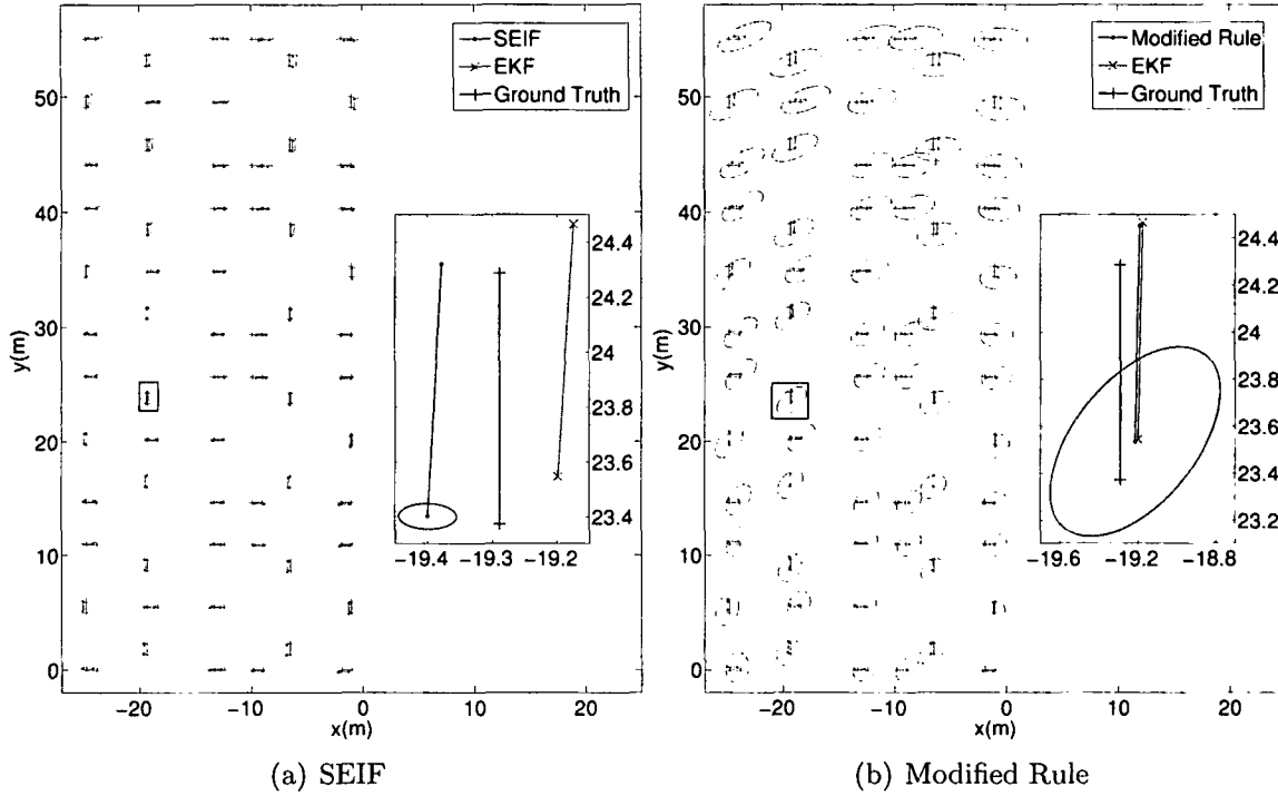
Figure 3-6: The final global maps for the (a) SEIF and (b) modified rule, along with the three-sigma uncertainty ellipses. We compare each to the map generated with the standard EKF, as well as the manually-measured ground truth hurdle positions. The SEIF maintains global feature estimates that are significantly overconfident as the uncertainty bounds do not capture the ground truth or the EKF estimates. The modified rule, meanwhile, yields estimates for absolute feature pose and uncertainty which are nearly identical to those of the EKF.
