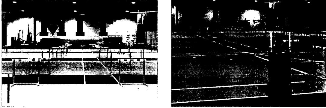
Figure A-1: The experimental setup for the hurdles dataset. The environment consists of 64 track hurdles positioned on the baselines of four adjacent tennis courts. The iRobot B21r robot is equipped with a laser scanner mounted near the base of the vehicle that provides measurements of range and bearing to the hurdle legs within its field-of-view. Note that the second laser scanner affixed at the top of the robot was not used during this experiment.
