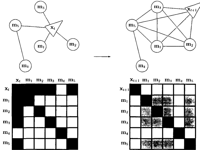
Figure 4-1: At time t , the robot observes four features, \{m_1, m_2, m_3, m_5\} , three of which are already active, while m_3 is passive. The update strengthens the shared information between vehicle pose and m_1, m_2 , and m_5 and adds a link to m_3 as we indicate on the left. The next time projection step forms a clique among the robot and these four features and populates the information matrix. The ESEIF sparsification strategy avoids this effect by controlling the number of active landmarks and, in turn, the size of this clique.
