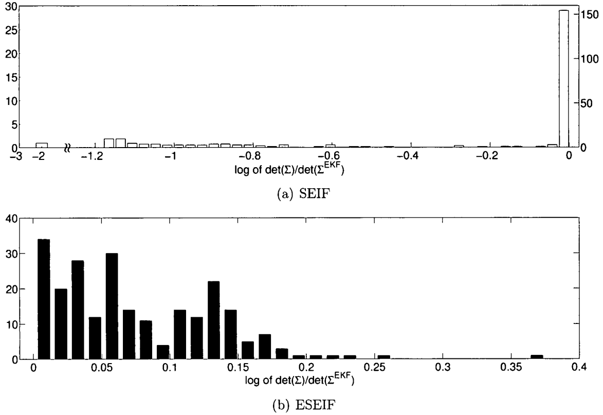
Figure 4-11: Histograms for the Victoria Park dataset that compare the relative (a) SEIF and (b) ESEIF uncertainty estimates to those of the EKF. We see that the ESEIF estimates remain conservative relative to the EKF and that the SEIF overconfidence persists, but is less severe.
