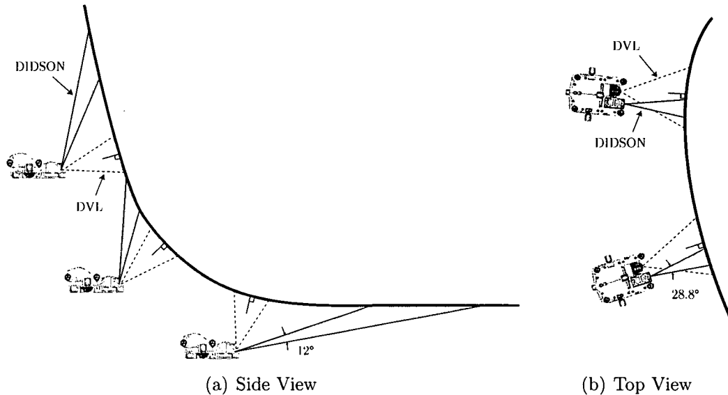
Figure 5-3: A schematic (not to scale) of hull-relative navigation in which the HAUV maintains a heading orthogonal to the hull surface at a fixed distance. The vehicle servos its pose, as well as the DVL pitch, based upon a planar model for the local hull geometry. The DVL orientation determines the DIDSON's pitch to achieve a suitable viewing angle.
