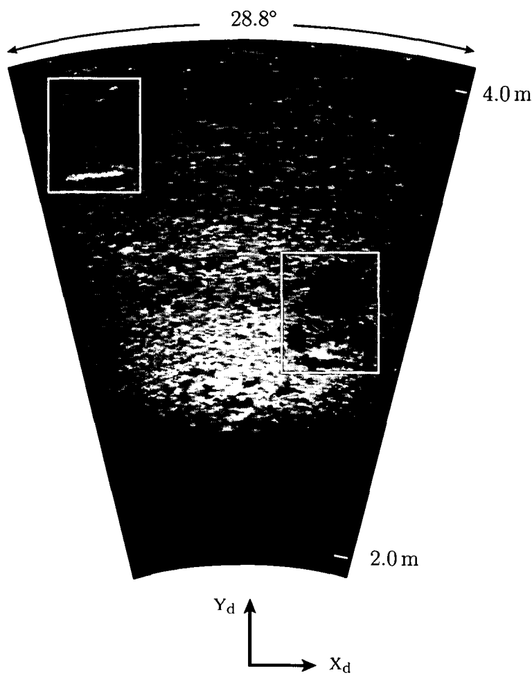
Figure 5-2: The DIDSON acquires two-dimensional acoustic intensity images that are a function of range and bearing that we show mapped into Cartesian space. Visible in the right side of the image is a 23 cm diameter cylindrical target and, on the left, a 50 cm rectangular feature. These targets represent the scale of features that we detect on the hull.
