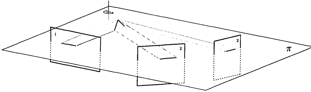
Figure B-2: Pairs of affine camera images are subject to the bas-relief ambiguity that describes the coupling between the scene's depth relief and the relative camera rotation. Under parallel projection, a large camera rotation about an axis that lies within a fronto-parallel plane and a shallow scene produces the same pair of images as a smaller rotation but larger depth relief. This effect gives rise to a one parameter family of transformations between affine camera pairs.
