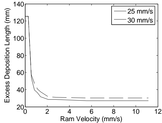
Figure 4: Ram retreating test data for the original extrusion mechanism.
