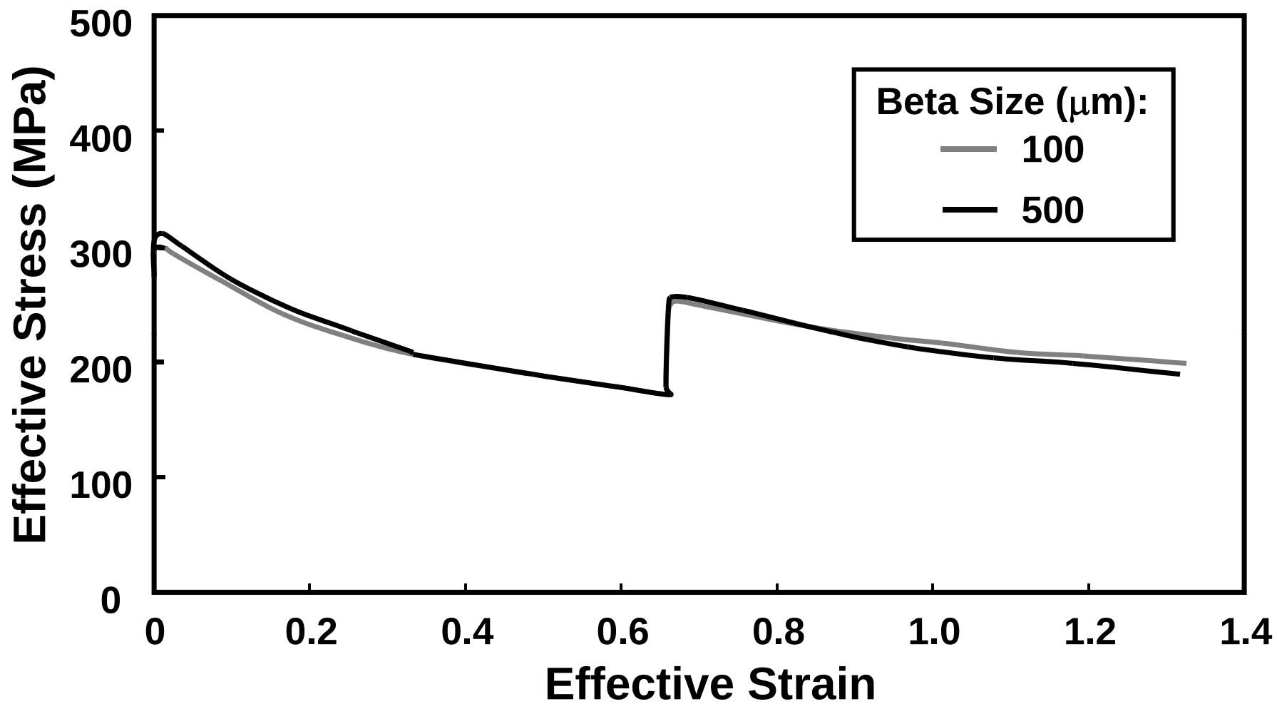
Figure 5. Effective stress-strain curves for compression-compression deformation at 815°C and an effective strain rate of 0.1 s -1 on specimens with two different beta grain sizes.
