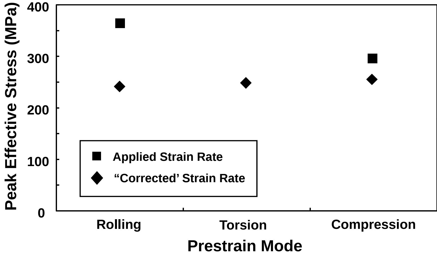
Figure 7. Peak stress during prestraining of Ti-6Al-4V. The data correspond to a temperature of 815°C; all data points were adjusted to a strain rate of 0.04 s -1 using a strain-rate sensitivity equal to 0.15.
