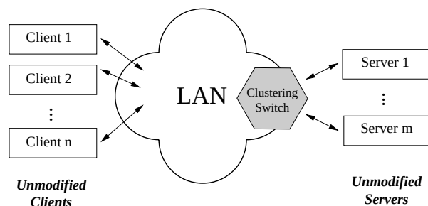
Figure 1: Layered clustering architecture. Clients, servers, and the client-server protocol are unmodified. The “clustering switch” is the only change, and it’s role is to add the clustering functionality by transparently translating some client requests into redirected server requests. The same role can be played by a collection of small intermediaries at the front-ends of the servers.
