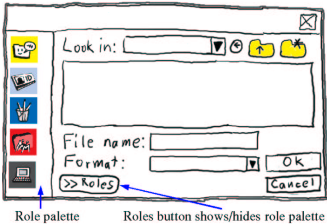
Figure 3: Role-aware file dialog box. The role palette on the left side chooses the role to browse. The “Roles” button hides and shows the role palette.
