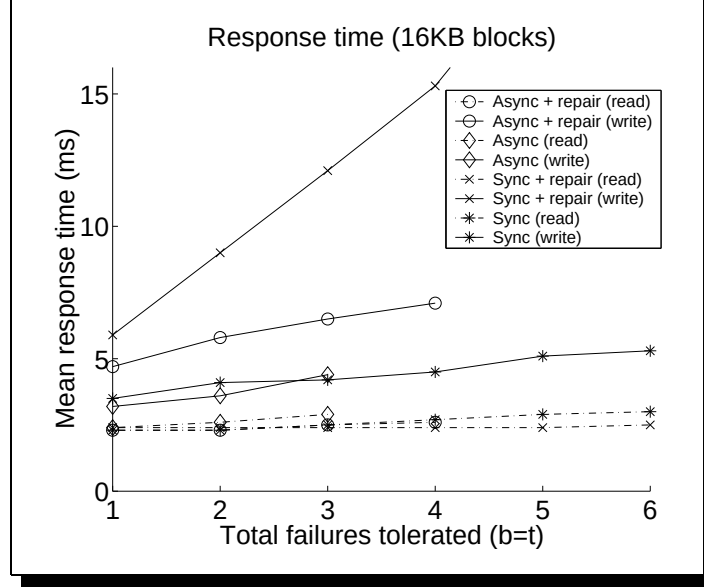
Figure 5: Response time of protocol family members. Mean response times of read and write operations of random 16 KB blocks are shown for the (asynchronous/synchronous, repair/non-repair) protocol family members with crash clients and Byzantine storage-nodes.
