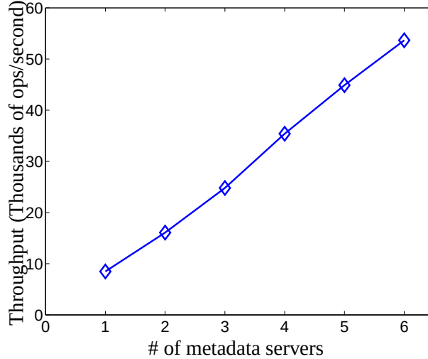
Figure 4: Metadata Servers vs Throughput. Throughput using the Harvard EECS workload scales linearly with respect to the number of Metadata Servers.
