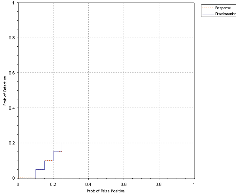
Figure 3. MAG G843/sling mogul probability of detection for response and discrimination stages versus their respective background alarm rate over all ordnance categories combined.
