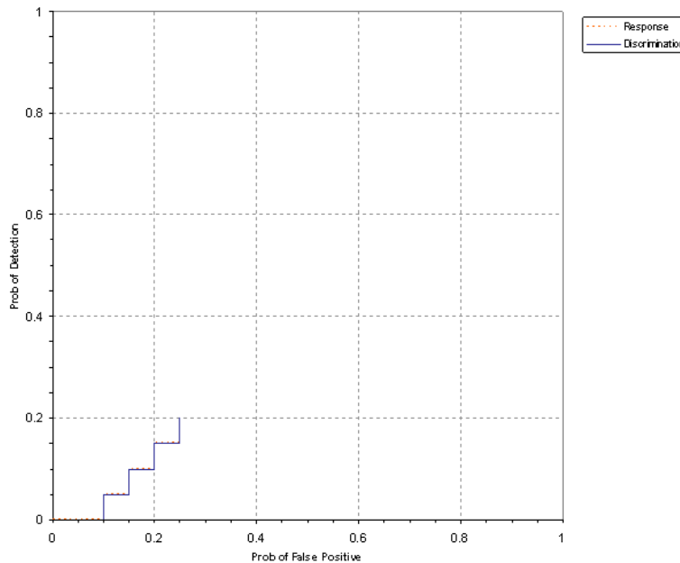
Figure 2. MAG G843/sling mogul probability of detection for response and discrimination stages versus their respective probability of false positive over all ordnance categories combined.
