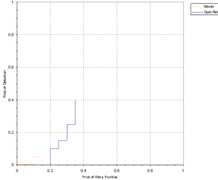
Figure 9. MAG G843/sling P_d^{\text{disc}} versus the respective P_{\text{fp}} for ordnance larger than 20 mm.
