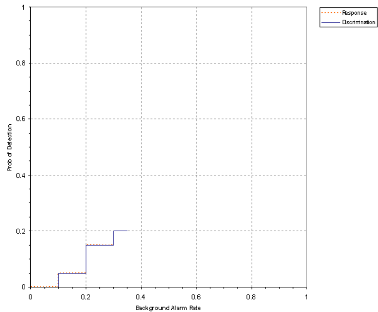
Figure 5. MAG G843/sling mogul probability of detection for response and discrimination stages versus their respective background alarm rate for all ordnance larger than 20 mm.
