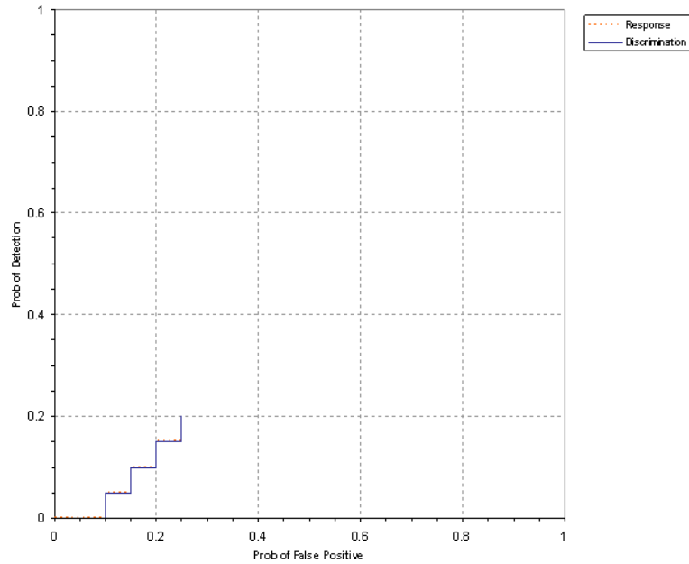
Figure 4. MAG G843/sling mogul probability of detection for response and discrimination stages versus their respective probability of false positive for all ordnance larger than 20 mm.
