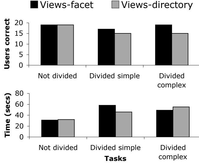
Figure 5: Dividing data. This graph shows the accuracy and time results for a set of tasks that asked reliability questions about data divided in different ways.
