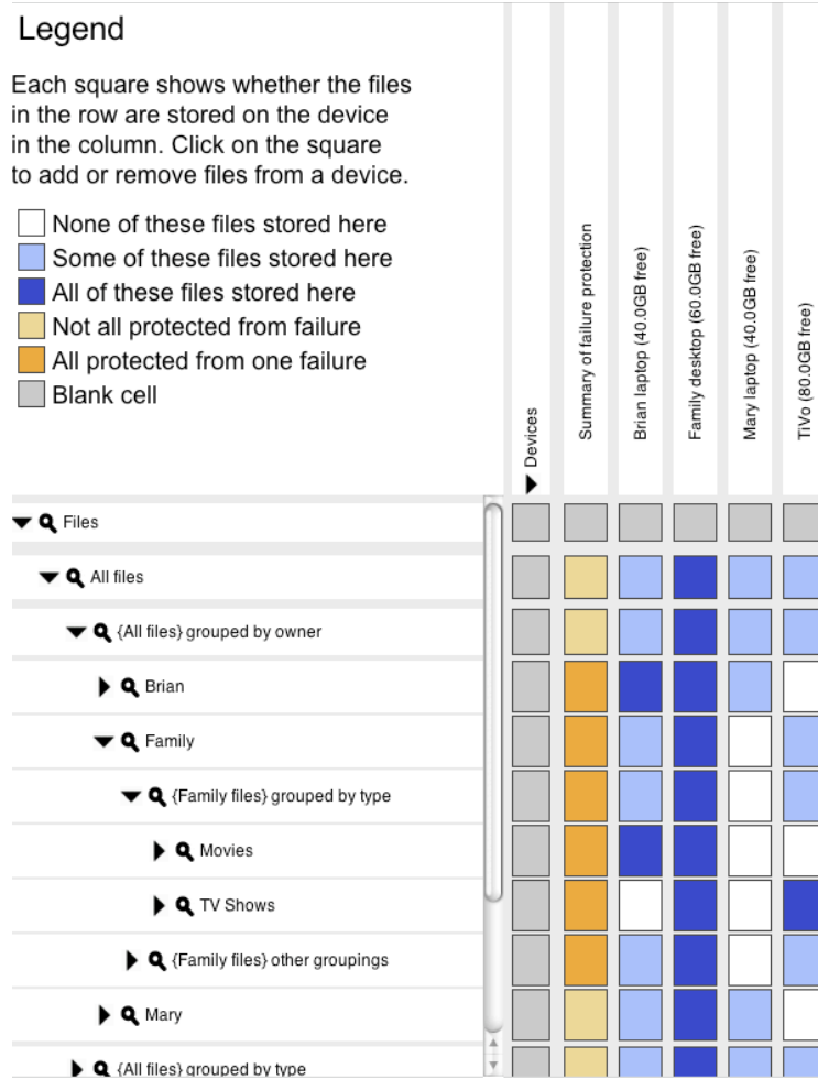
Figure 2: View manager interface. A screen shot of the view manager GUI. On the left are files, grouped using faceted metadata. Across the top are devices. Each square shows whether the files in the row are stored on the device in the column.
