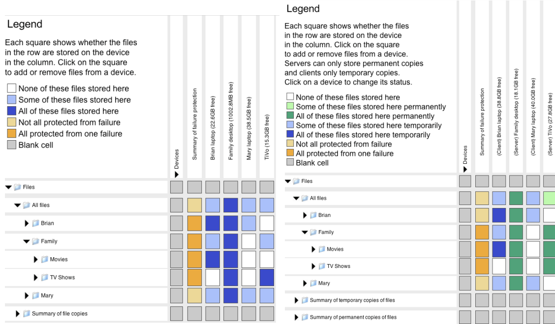
Figure 3: Comparison interfaces. On the left is a screenshot of the views-directory interface, on the right the volumes interface.
