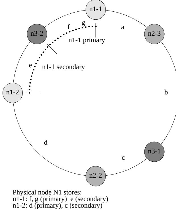
Figure 3. An example ring with three physical nodes. Items a, b, ..., g, are data items mapped to their locations in the ring.
