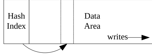
Figure 5. The FAWNDB back-end storage format. The index and data areas are separate, and all data inserts are sequentially written to the end of the data area, ensuring log-like performance.
