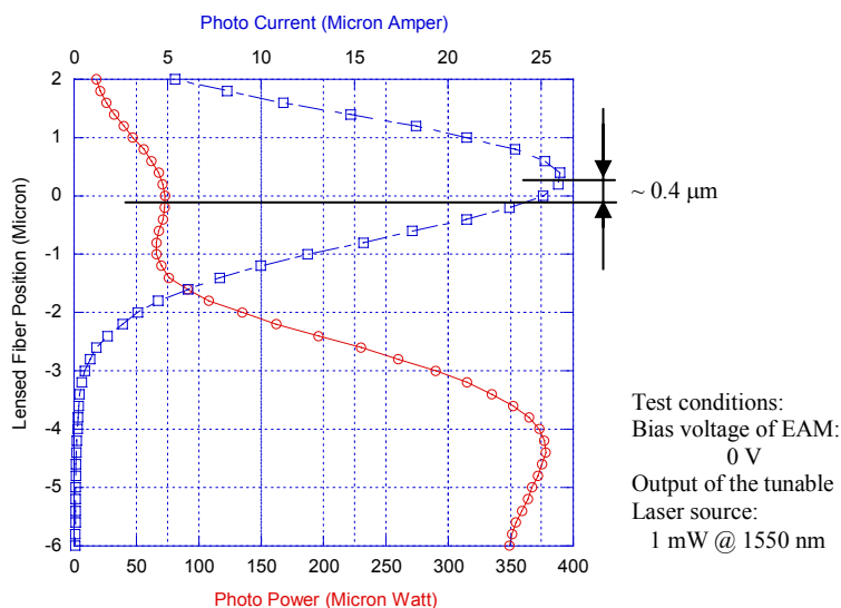
Figure 5: The photo current and photo intensity curves of DCW EAM
