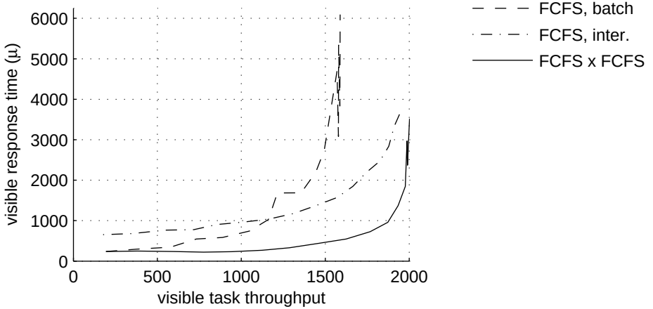
Figure 6.15: The relationship on batchactive usage of \text{FCFS} \times \text{FCFS} , interactive usage of FCFS, and batch usage of FCFS between visible throughput and mean visible response time as the number of users was varied from 1 to 16. Both axes are dependent axes; the horizontal axis indicates visible task throughput while the vertical axis indicates mean visible response time. The number of users was varied while other parameters were held constant. The more the batchactive curve is below and to the right of the other curves, the better its performance, as that indicates better visible throughput at better mean visible response time. \text{FCFS} \times \text{FCFS} always provides better pairs of visible throughput and mean visible response time. At a visible throughput of 1,500, the visible response time of \text{FCFS} \times \text{FCFS} is over 3 times better than interactive FCFS and over 6 times better than batch FCFS. Note that this particular improvement was achieved with a different number of users for the different scheduling configurations. That is, for any visible task throughput or any visible response time, it is likely that a different number of users resulted in that performance for the different scheduling configurations. The setting of this independent variable may be found by examining Figures 6.10 and 6.14 for number of users v. mean visible response time and v. visible throughput, respectively.
