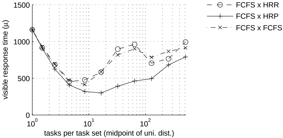
Figure 6.39: The effect of the number of tasks per task set on batchactive usage of \text{FCFS} \times \text{HRR} , batchactive usage of \text{FCFS} \times \text{HRP} , and batchactive usage of \text{FCFS} \times \text{FCFS} for mean visible response time. Each set of three configurations was run with a different upper bound on the uniform distribution determining the number of tasks per task set for each user; the lower bound was held constant at 1. Other parameters were held constant. The number of tasks per task set is a uniform random variable and shown on the horizontal axis is the average of its lower and upper bounds. The saddle points at the horizontal axis value of 128 is within confidence intervals (not shown). FCFS \times HRP performs significantly better in the middle region of this graph, exhibiting greater robustness. (This graph is log-linear.)
