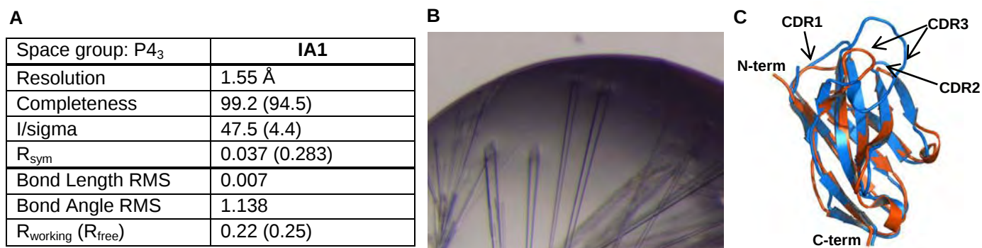
Figure 7. Crystal structure of IA1 llama V HH antibody. The structure of antibody IA1 was determined to a resolution of 1.55 Å. Data were collected at the Advanced Photon Source, beamline 23 ID-B. Data collection and refinement statistics (for the current stage of refinement) are given in A. Values in parenthesis reflect the highest resolution shell of data. RMS = root mean square deviation. (B) Rod-like crystals (75x75x500 um) formed in 30% PEG8000, 0.2M ammonium sulfate, 0.1 M MES, pH 6.0. (C) Cartoon representation of IA1 (blue) overlaid with the N-terminal Ig domain of the C225 heavy chain (from PDB 1yy8). Differences between the two structures reside chiefly in the complementarity determining region (CDR) loops. Particularly, CDR3 is much longer in IA1 and folds against the surface of the Ig domain.
