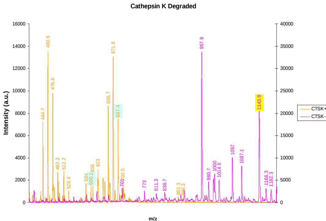
Figure 7: Mass spectrometry of the peptide consisting of the cathepsin K protease site (CTSK) before and after cleavage with the protease.
