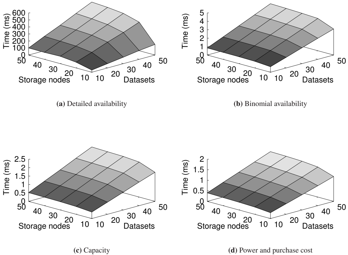
Figure 3.2: System model performance – These figures show the performance of the individual system models as a function of the size of the storage system being evaluated. The storage system sizes range between 10 and 50 storage nodes with 10 to 50 datasets in the system. There is always one workload and one client for each dataset.
